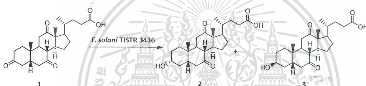
Scheme 1 Biotransformation of dehydrocholic acid by F. solani TISTR 3436
