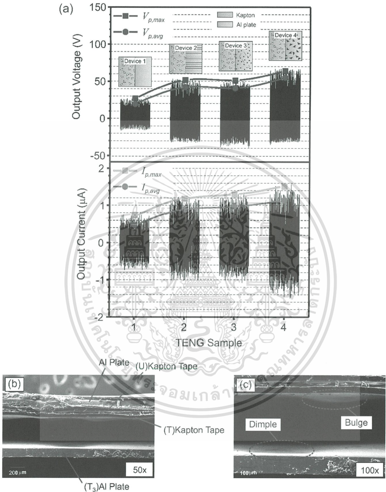
Figure 8. (a) Summation of the output voltage and current results obtained from four optimum TENGs. Cross-sectional SEM images of device 4 with magnifications of (b) 50× and (c) 100×.
