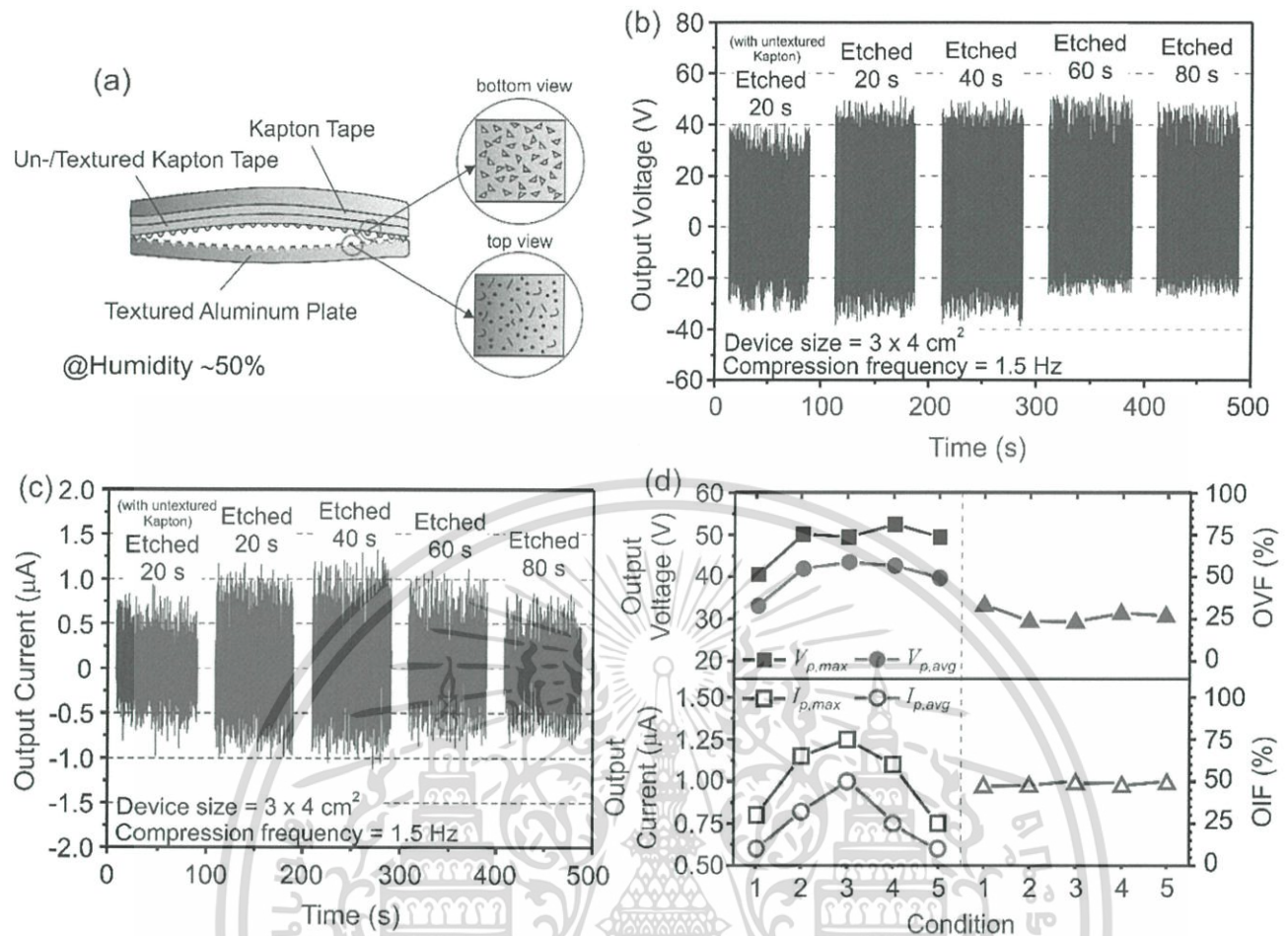
Figure 6. (a) Structure of the TENG device with rubbing between the textured Kapton tape and textured Al plate etched with \text{FeCl}_3 at various etching times. The insets show the shape of roughness generated on the material surfaces. (b) Output voltage and (c) output current waveforms of the TENGs at various etching times from 20 to 80 s. (d) The averaged maximum positive output voltage ( V_{p,max} ), the averaged positive output voltage ( V_{p,avg} ), the averaged maximum positive output current ( I_{p,max} ) and the averaged positive output current ( I_{p,avg} ) in each condition (left-hand side figure). The graph on the right-hand side shows the calculated output voltage fluctuation (OVF) and the calculated output current fluctuation (OIF) of the TENGs.
