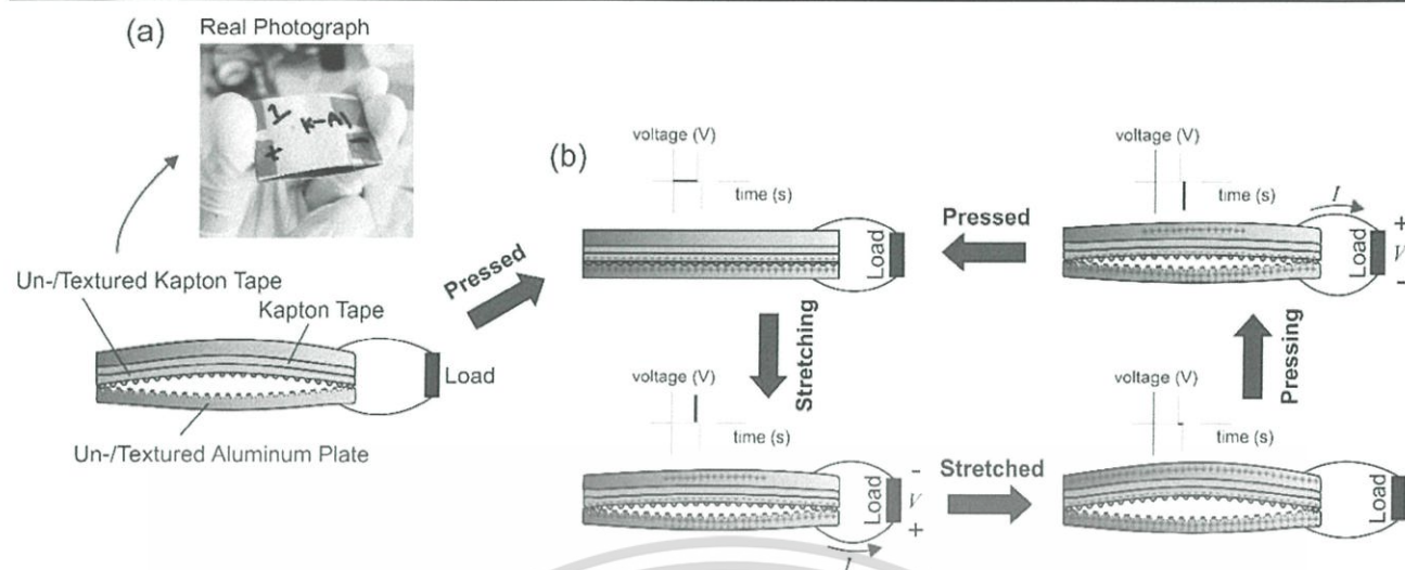
Figure 3. (a) General structure of the TENG used in this work (left-hand side of figure). The Kapton tape is rubbing directly against the Al plate. Here, the Al plates located on the top and bottom structures act as device electrodes. (b) Basic working mechanism of the TENG (right-hand side figure) with a single-rubbing pair contact mode. The TENG generates the triboelectric current I and triboelectric potential V .
