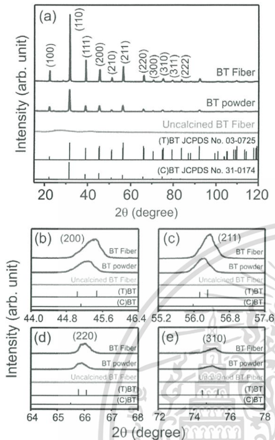
Fig. 1. (a) Room temperature XRD patterns of BT fiber, BT powder and uncalcined BT fiber. The enlarged XRD patterns are in the range 2\theta of (b) 44.0\text{--}46.4^\circ , (c) 55.2\text{--}57.6^\circ , (d) 64\text{--}68^\circ and (e) 72\text{--}78^\circ . (For interpretation of the references to color in this figure legend, the reader is referred to the web version of this article).
