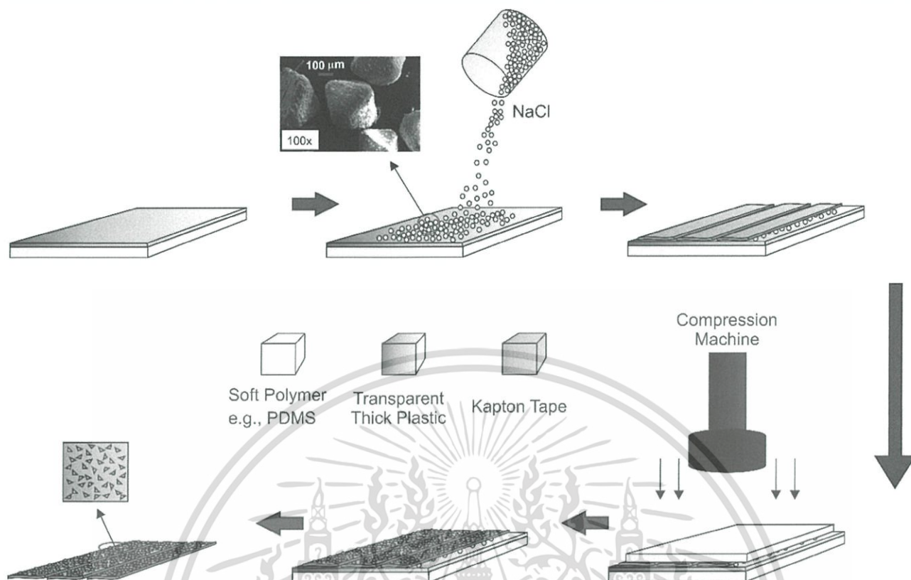
Figure 1. Schematic diagram of the cold compression (CC) technique for fabricating the texture of roughness on the material surface. Solid salt (NaCl), which has an averaged particle size of around 200\ \mu\text{m} , was used to create the texture.
