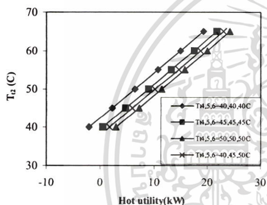
Figure 7: Hot utility and target temperature of case 3
