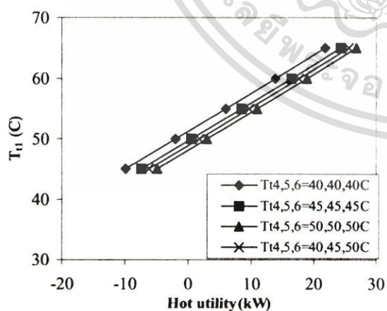
Figure 5: Hot utility and target temperature of case 1
