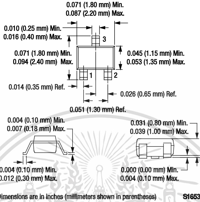
Figure 7. SC-70 Package Dimension Drawing
