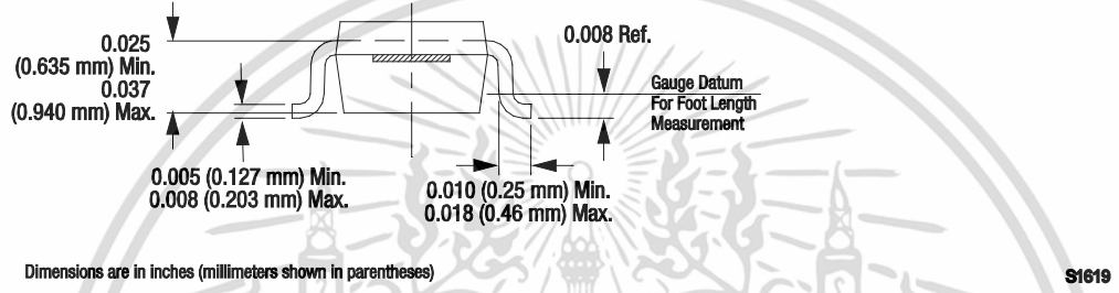
Figure 13. SOD-323 Package Dimension Drawing
