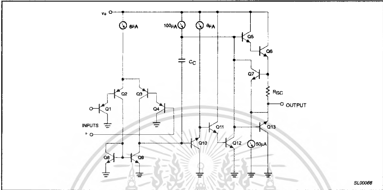
Figure 2. Equivalent Circuit
