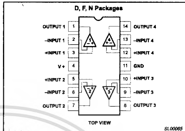
Figure 1. Pin Configuration
