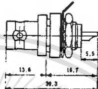
Outside-insulating connector Fig.27
