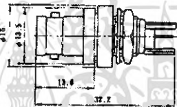
Outside-insulating connector Fig.27
