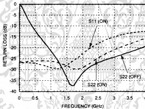
Return Loss
