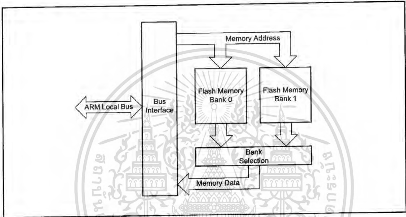
Figure 18: Simplified Block Diagram of the Memory Accelerator Module
