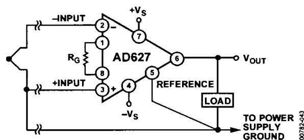
Figure 45. Ground Returns for Bias Currents with Thermocouple Inputs
