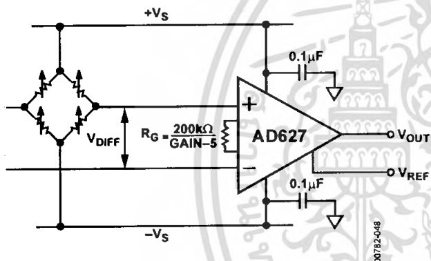
Figure 50. Classic Bridge Circuit
