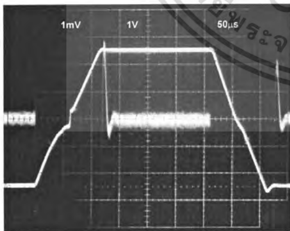
Figure 19. Large Signal Pulse Response and Settling Time, G = -10 , R_L = 20\text{ k}\Omega , C_L = 100\text{ pF} ( 1.0\text{ mV} = 0.01\% )
