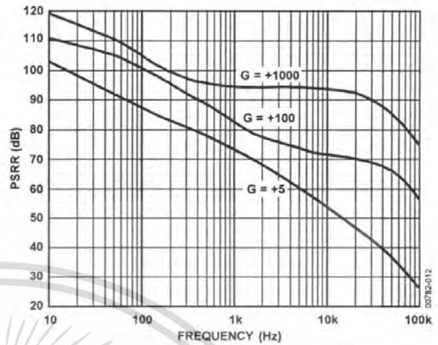
Figure 14. Positive PSRR vs. Frequency, ±5 V
