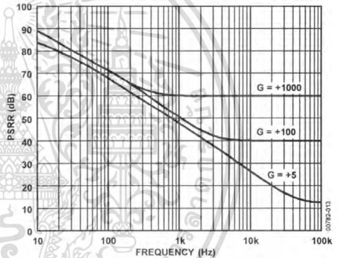
Figure 15. Negative PSRR vs. Frequency, ±5 V
