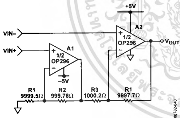
Figure 42. 0.1% Resistor Mismatch Example
