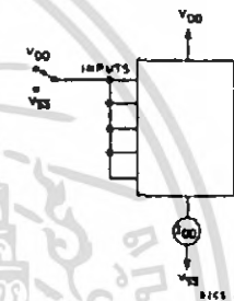
Fig. 10 - Quiescent device current.
