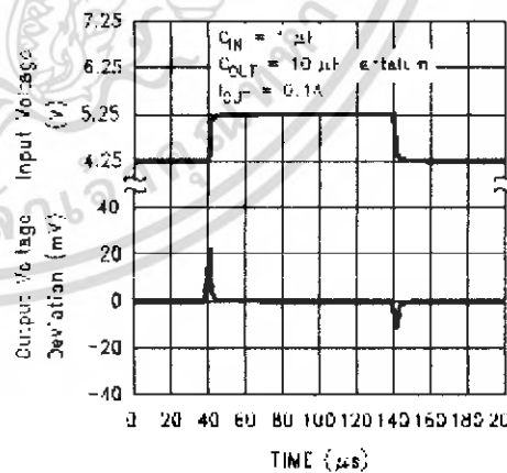
LM1117-2.85 Line Transient Response
