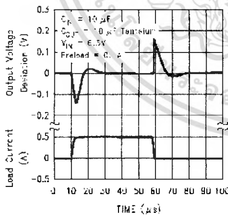
LM1117-5.0 Load Transient Response
