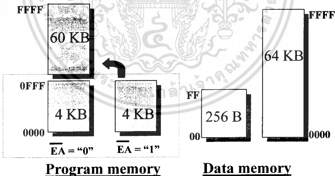
AT89C51 Memory system
