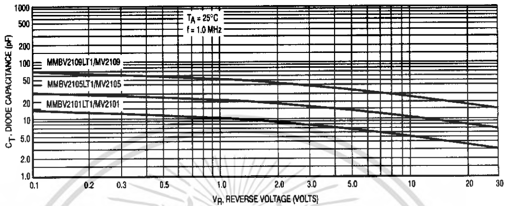
Figure 1. Diode Capacitance versus Reverse Voltage
