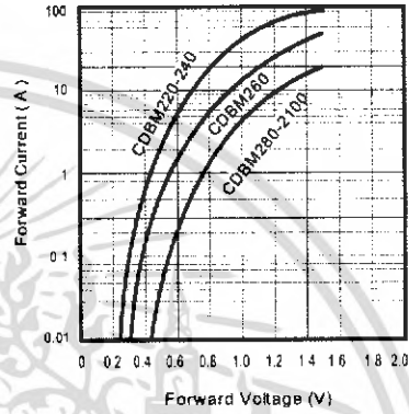
Fig.2 - Forward Characteristics
