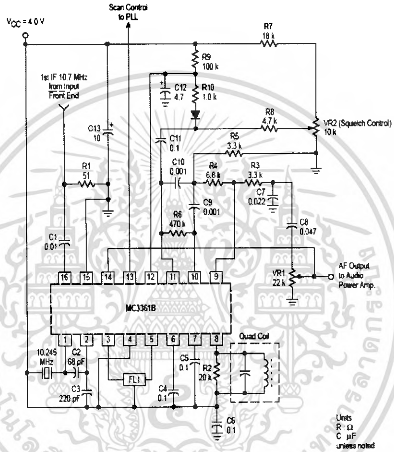
Figure 10. Simplified Application
