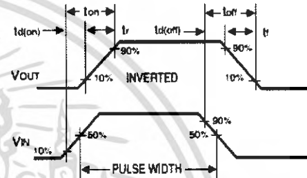
Figure 12. Switching Waveforms
