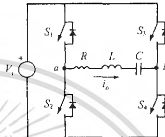
Fig. 1. Full-bridge series resonant inverter.
