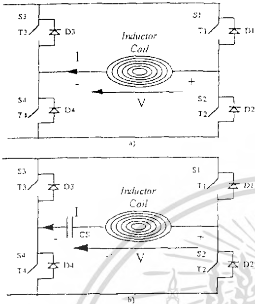
Fig. 1 Full-bridge topology for constant-frequency control of induction heating appliance. a) Non-resonant topology. b) Series-resonant topology
