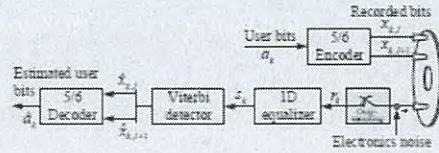
Fig. 2 Block diagram of the SRTR technique combined with the proposed rate-5/6 2D modulation code in a staggered BPMR system.
