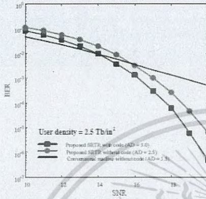
Fig. 7 The comparison of BER performance in different systems at the UD of 2.5 Tb/in 2 .
