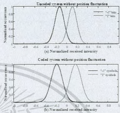
Fig. 5 Histogram of the normalized received intensities of the (a) un-coded and (b) coded systems without position fluctuation.
