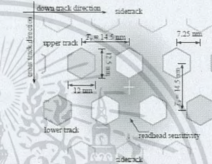
Fig. 1 Configuration of the proposed single-reader/two-track reading (SRTR) technique at the AD of 3.0 \text{ Tb}/\text{in}^2 under the read-head sensitivity response that was positioned between the desired upper and lower tracks.
