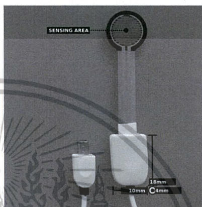
Fig. 1: Example of a Type 3 force sensor.
