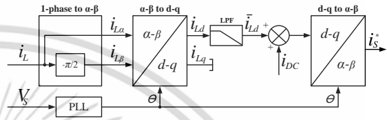
Fig.3 Reference source current generation using a single-phase synchronous d-q reference frame.
