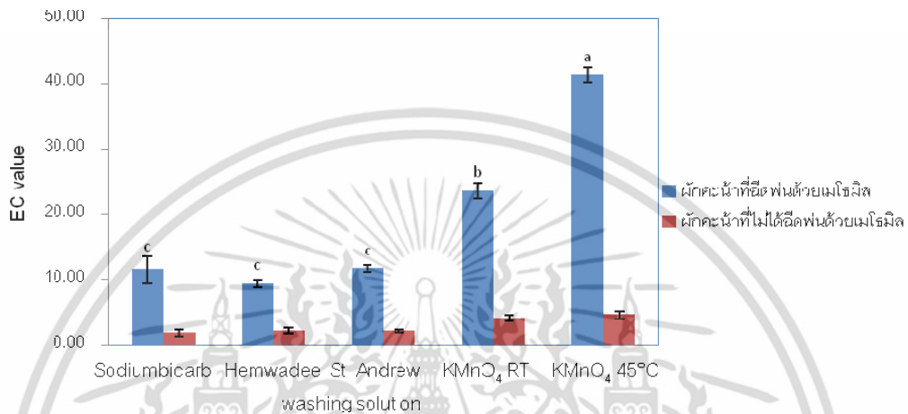
Figure 4 Electrical conductivity value of washing solution
