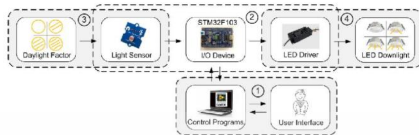
Fig.2 System overview
