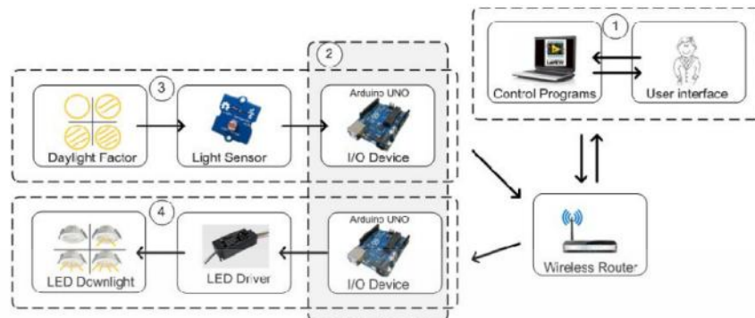
Fig.1 System overview
