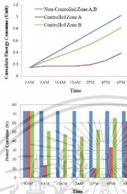
Fig.13 (a)Cumulate Energy consume (b)Power Consume
