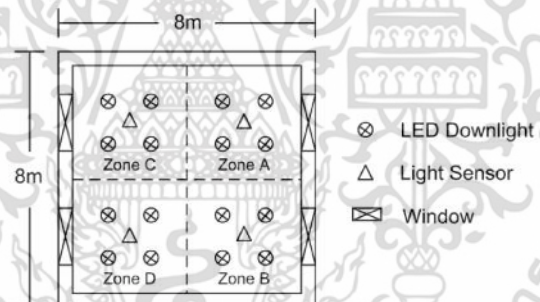
Fig.2 Room configurations and set up for Simulation
