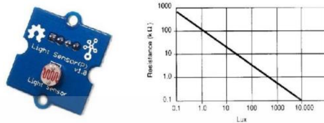
Fig.8 (a) Light Sensor (b) Resistance as illuminance
