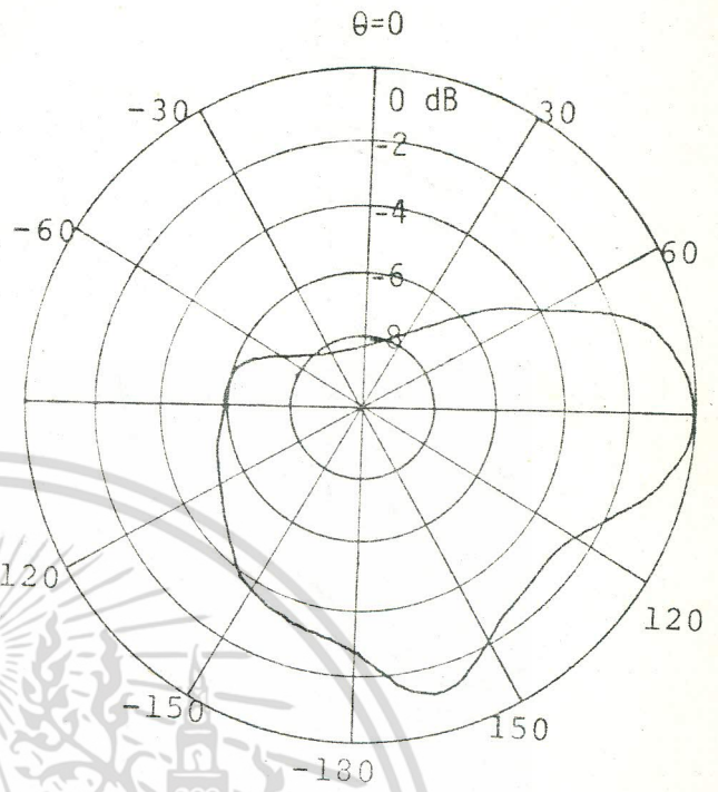
(ข) C_\lambda = 0.187
