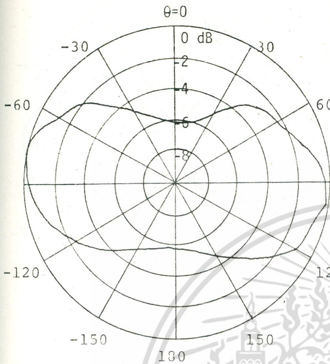
(จ) C_\lambda = 0.197
