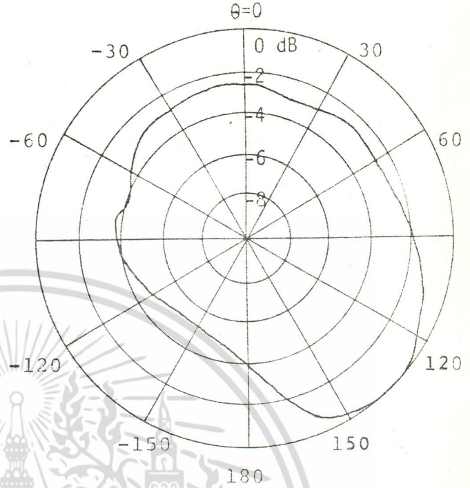
(ข) C_\lambda = 0.208
