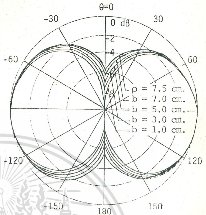
(ข) C_\lambda = 0.1
