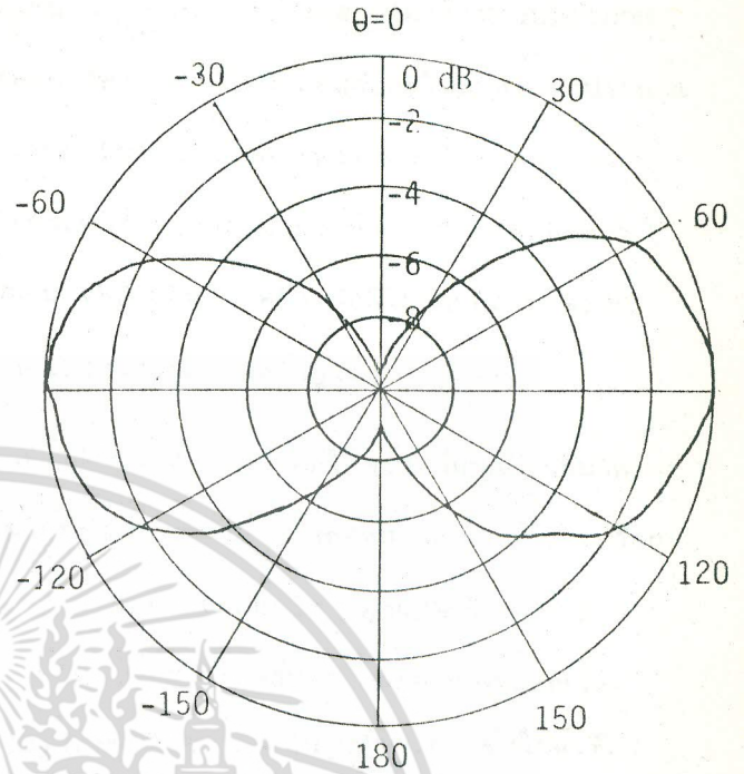
(ก) C_\lambda = 0.199
