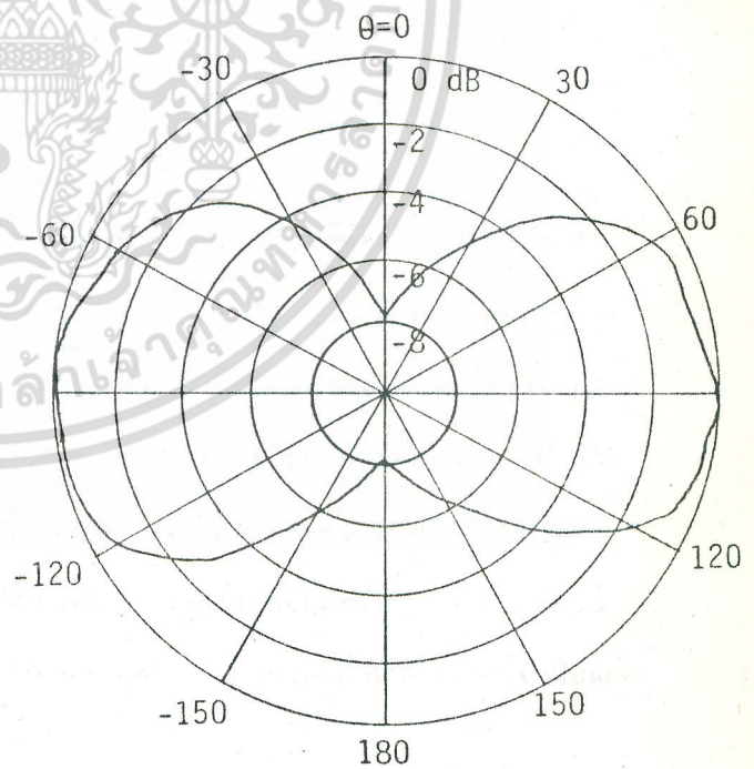
(ก) C_\lambda = 0.199
