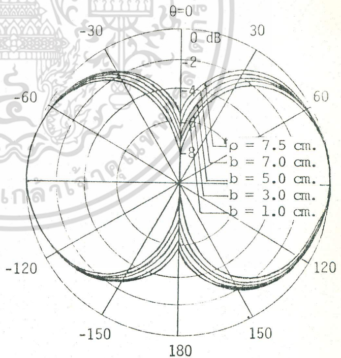
(ง) C_\lambda = 0.25
