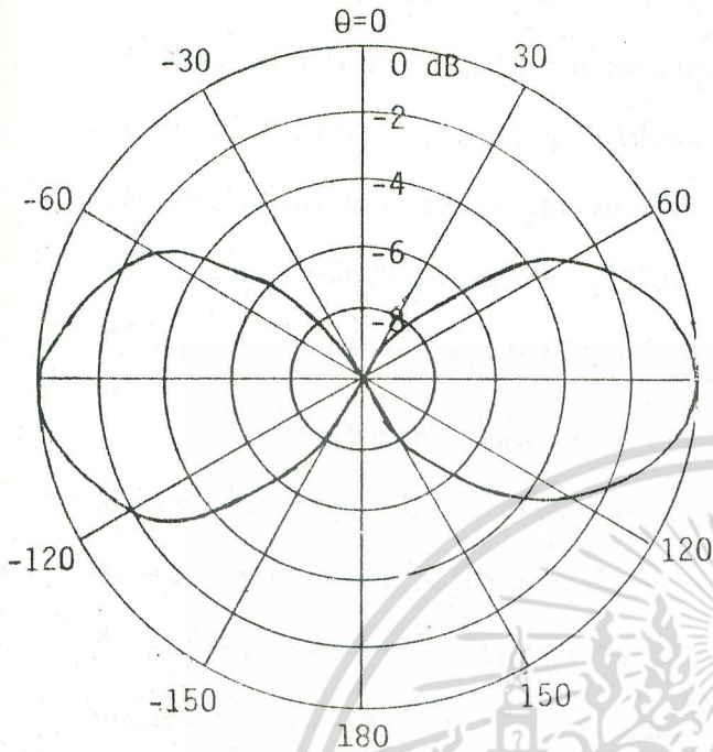
(จ) C_\lambda = 0.197
