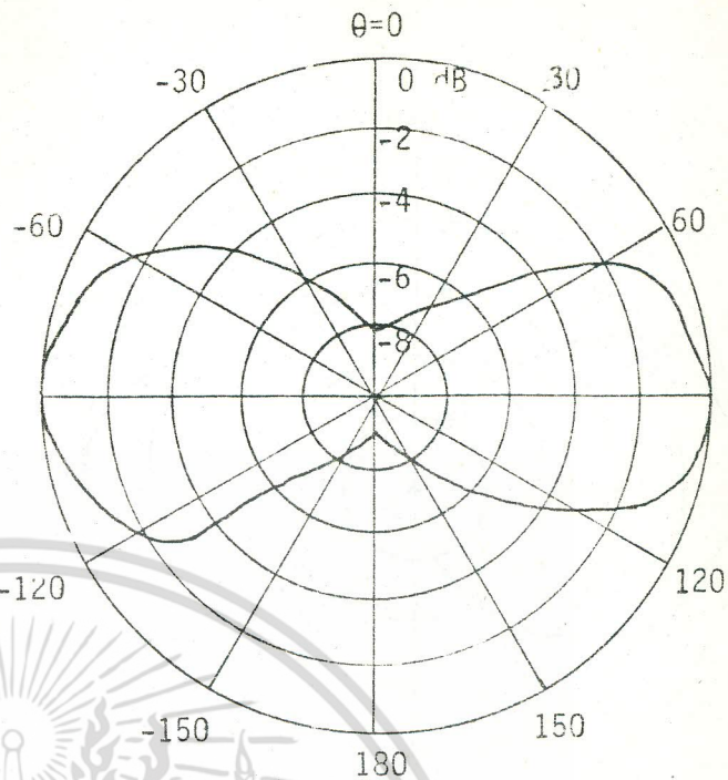
(ข) C_\lambda = 0.187
