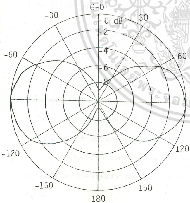
(ข) C_\lambda = 0.203
