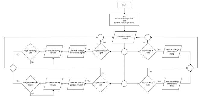
Fig. 7. Flowchart show PlayerController Script
