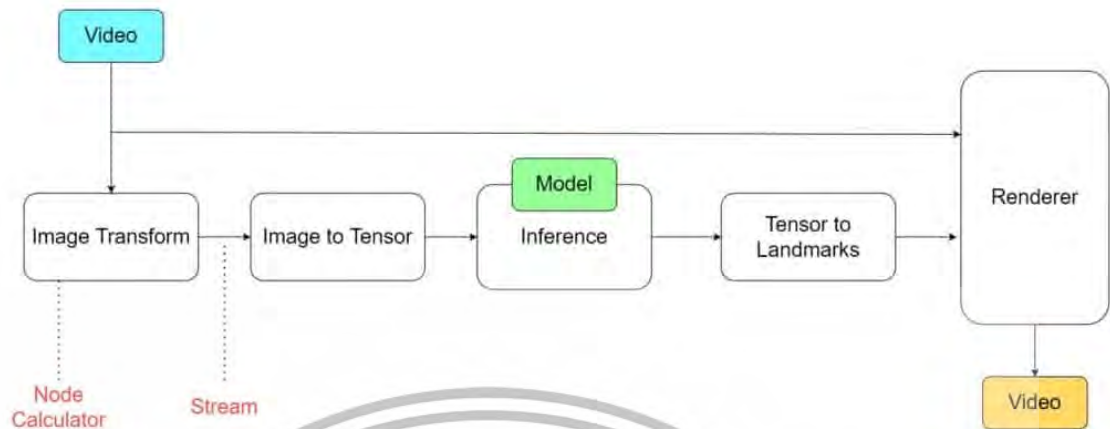
Figure 2.1 MediaPipe Solution Graph
