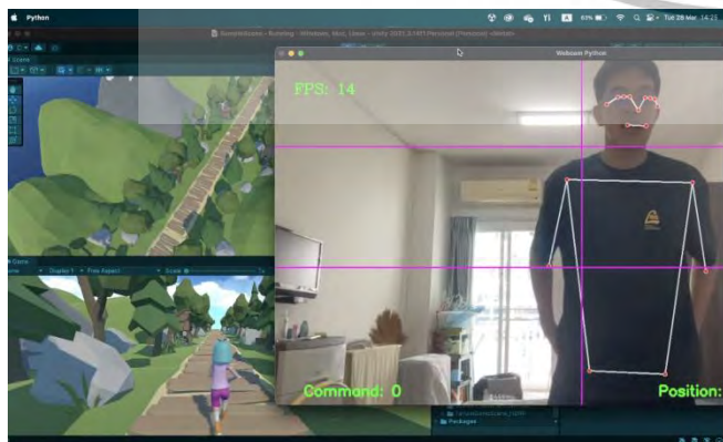
Fig. 2. Connection between MediaPipe to Unity
