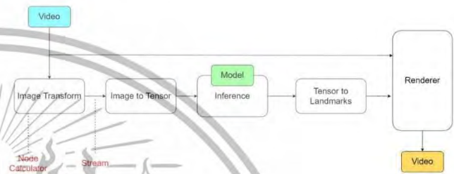
Fig. 1. MediaPipe Solution Graph
