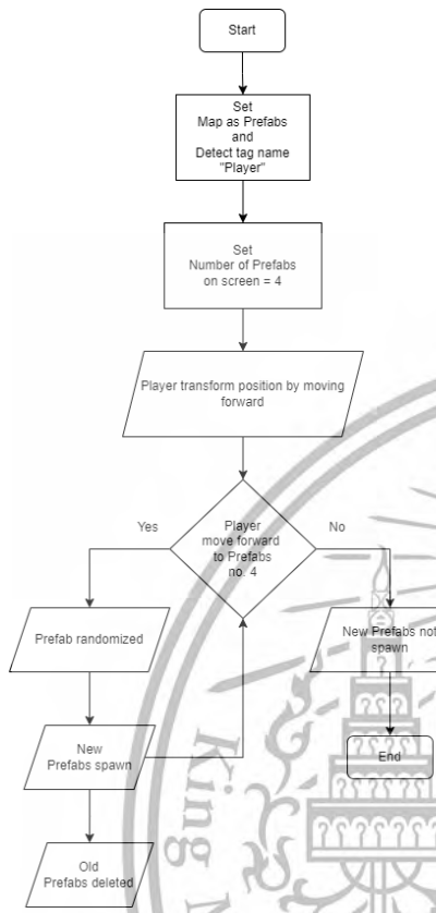
Fig. 9. Flowchart show MapSpawning Script
