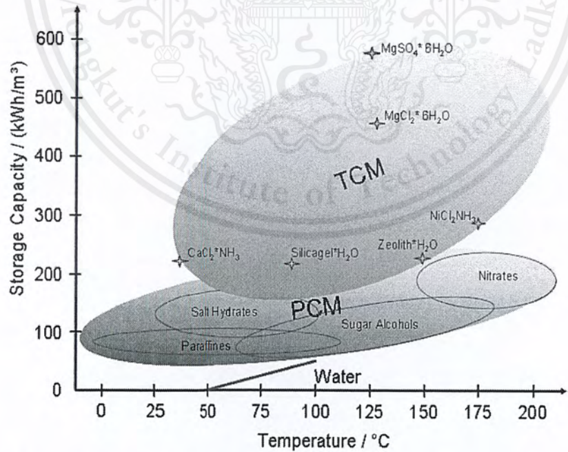
Figure 6 The ability to store heat energy with temperature range used to change the phase [5].
