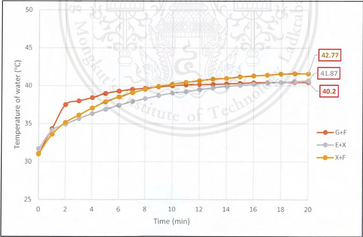
Figure 37 Graph between temperature of water in each mixtures and time (Part 2)
