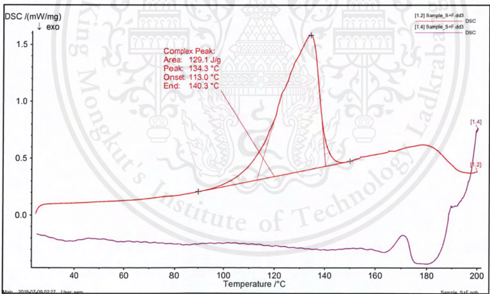
Figure 16 DSC curve of the sucrose - fructose system
