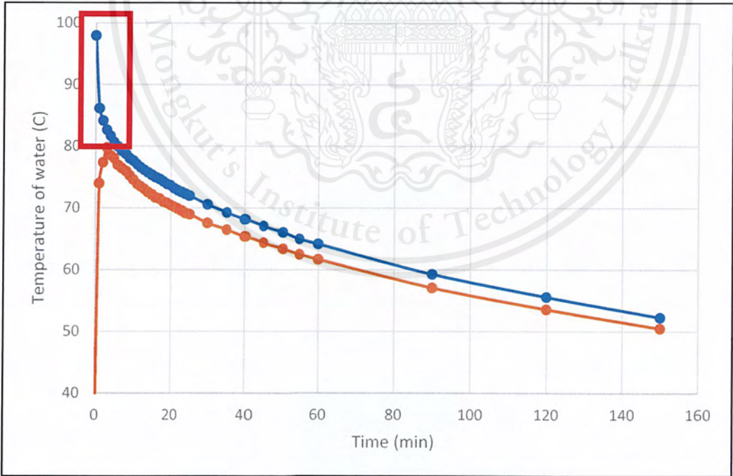
Figure 31 Graph between temperature and time of E+X (Part 1)
