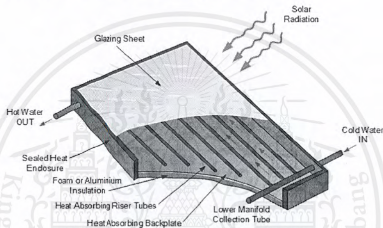
Figure 2 Schematic diagram of a Flat plate collectors
