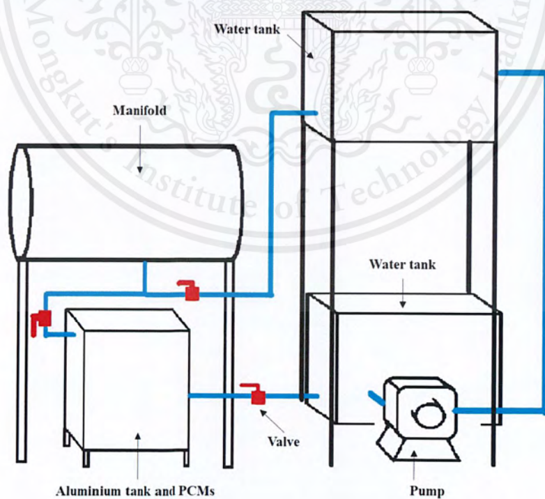
Figure 8 Thermal energy storage system
