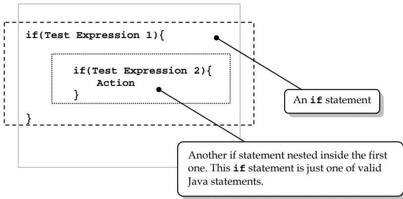
Figure 98: An example nested if statement
