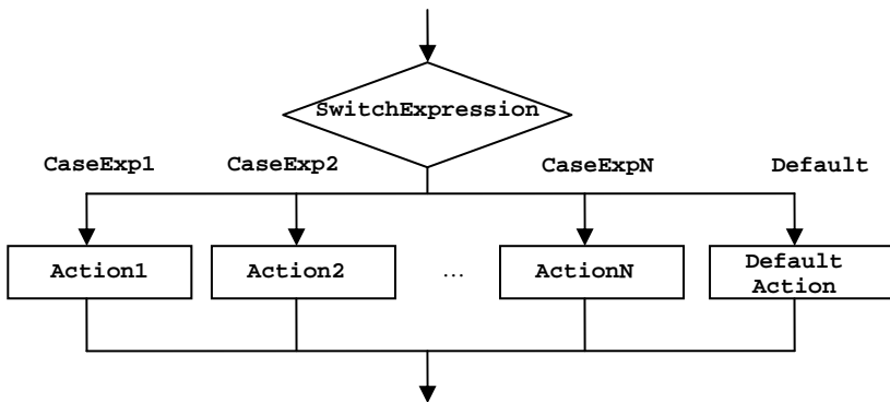
Figure 107: A flowchart representing a switch construct
