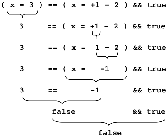
Figure 53: Order of operations in evaluating (x=3)==(x+=1-2)&&true
