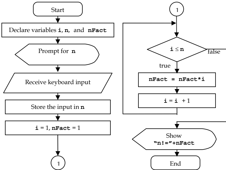
Figure 33: Flowchart of program calculating the factorial of a manually-input integer value
