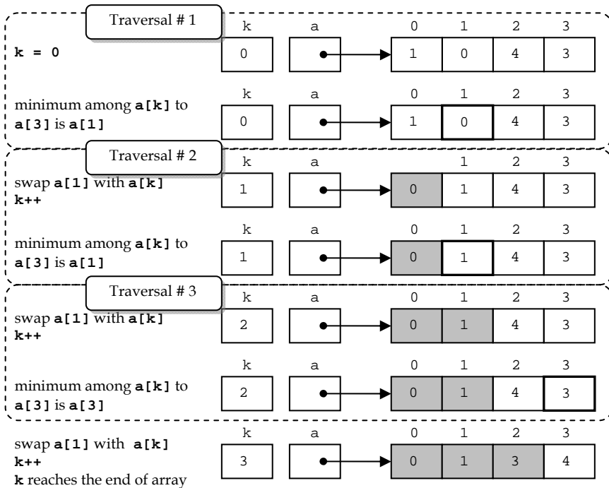
Figure 157: An example of performing the selection sort on an array. Each traversal only traverses the portion of the array that is not shaded.
