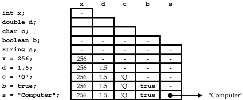
Figure 39: Storing values into variables
