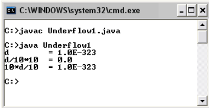
Figure 62: A demonstration of cases when underflow occurs
