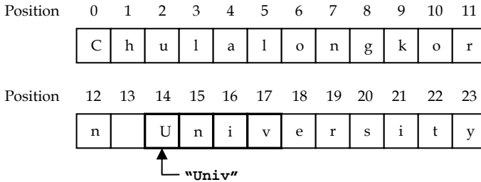
Figure 76: Finding Strings in another String
