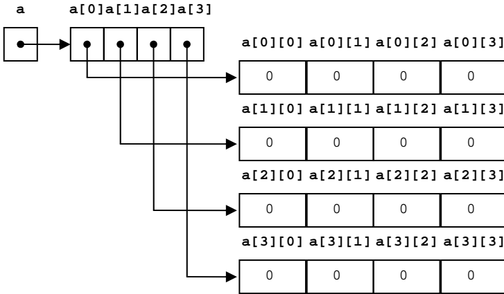
Figure 159: An array of arrays of int
