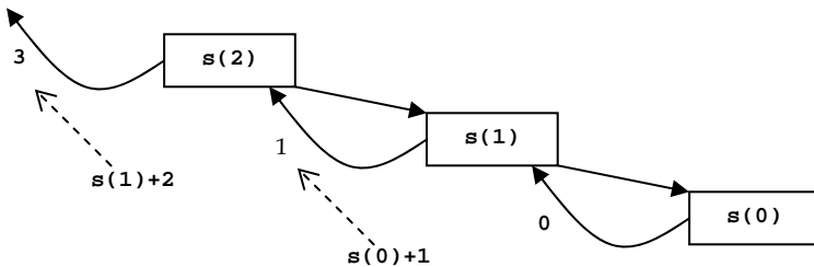
Figure 162: Finding s(n)=s(n-1)+n where n=2 recursively
