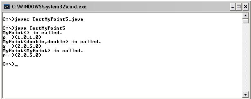
Figure 182: Demonstration of using overloaded constructors
