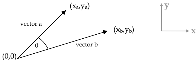
Figure 130: Two vectors in the Cartesian coordinate
