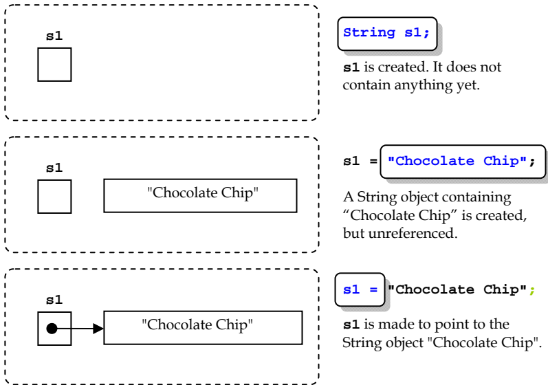
Figure 68: Declaration and assignment of a String object
