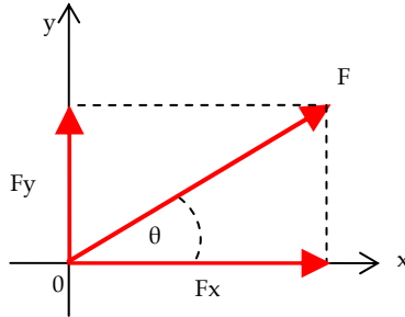
Figure 85: Decomposition of a vector F into F_x and F_y
