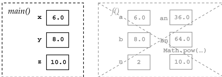
Figure 137: Illustration of variables when f() is invoked (Step4)
