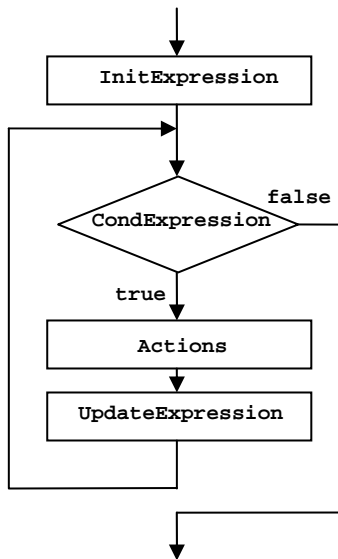
Figure 119: A flowchart representing a for statement
