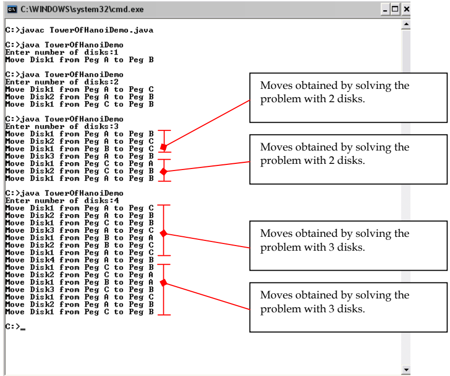
Figure 169: Solutions to the Towers of Hanoi puzzle
