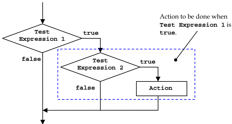
Figure 97: A flowchart associated with a nested if construct
