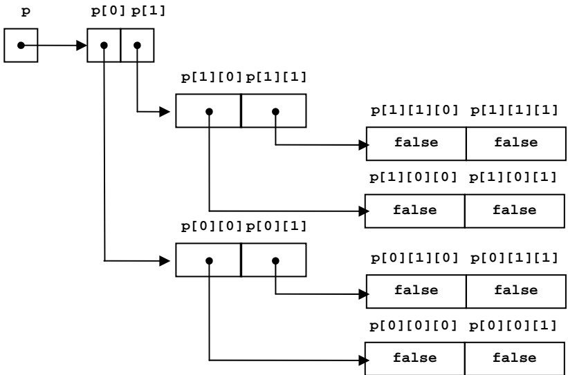
Figure 160: A three dimensional array of boolean
