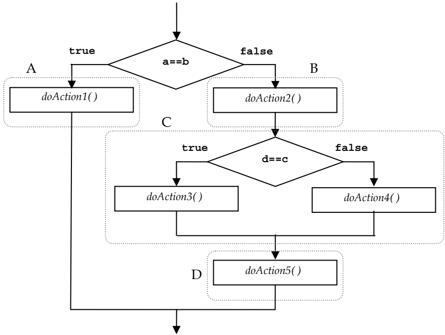
Figure 99: A flowchart representing a portion of a program
