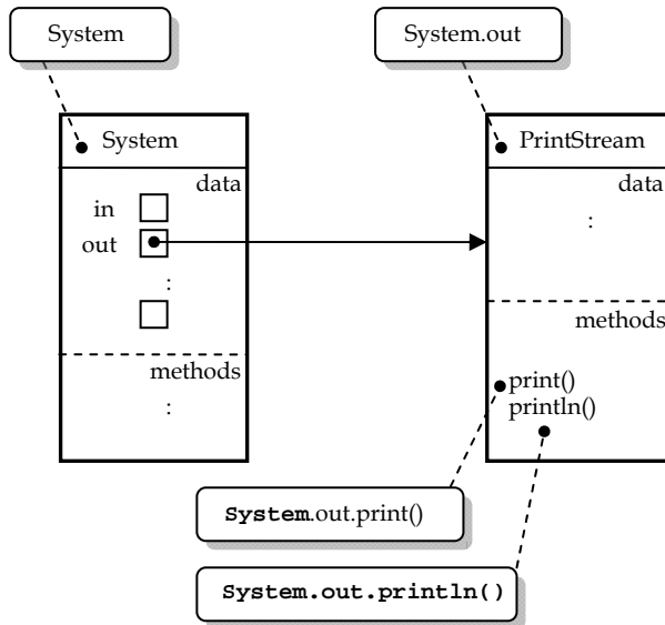
Figure 70: An abstract representation classes, objects, and methods involving in System.out.print() and System.out.println()
