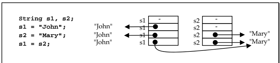
Figure 40: Reassigning a String variable
