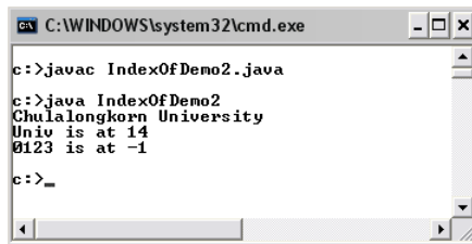
Figure 75: Demonstration of using lastIndexOf()
