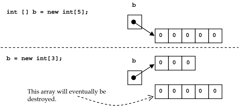
Figure 149: Assigning a new array to a variable
