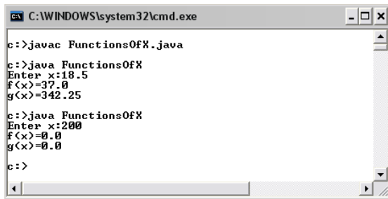
Figure 96: A program that use an if-else construct to choose which functions to be calculated
