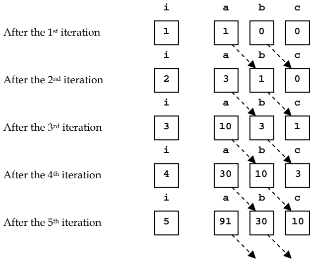
Figure 164: How variables change when the loop keeps iterating
