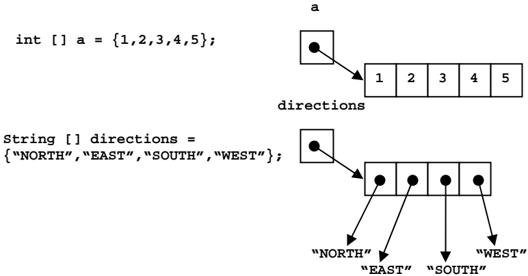
Figure 148: Illustration of some usage of initializer lists
