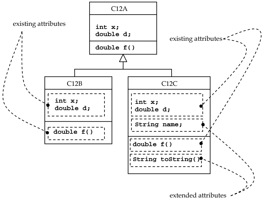
Figure 188: Class inheritance diagram relating C12A, C12B, and C12C
