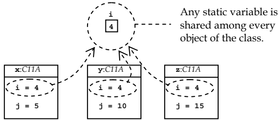
Figure 178: A diagram showing three objects of the C11A class and the values of their instance and class variables
