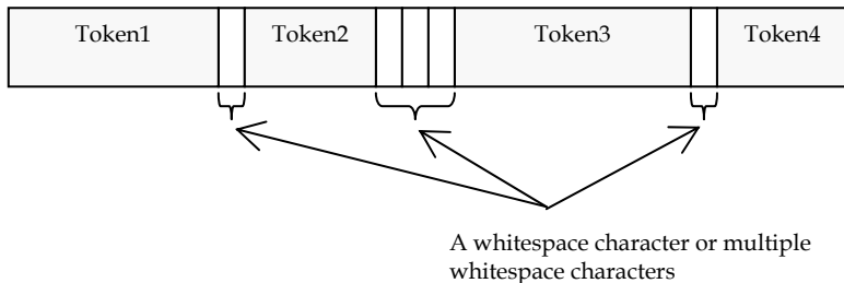
Figure 87: The default pattern used by a Scanner object
