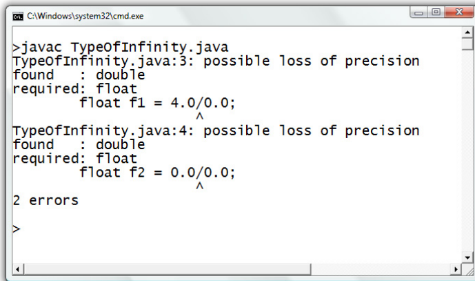
Figure 65: Compilation errors due to data type mismatch in the cases when numbers are divided by zeros
