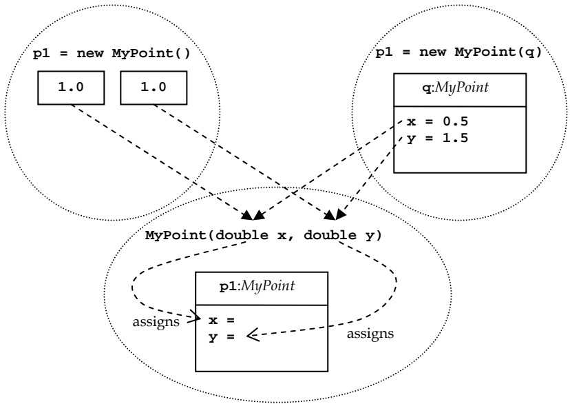
Figure 184: Re-using the detailed constructor
