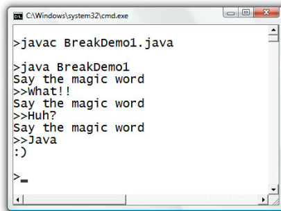
Figure 123: Demonstration of using the break statement
