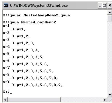
Figure 126: Another example of nested loops in action
