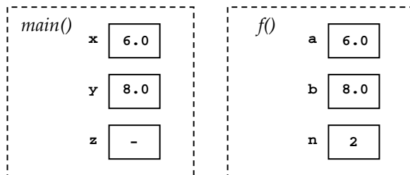
Figure 135: Illustration of variables when f() is invoked (Step2)
