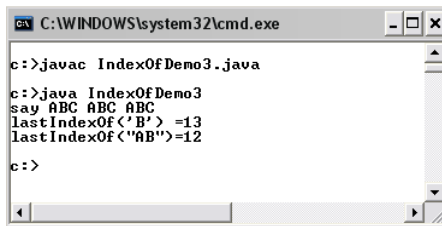
Figure 77: Demonstration of using lastIndexOf()
