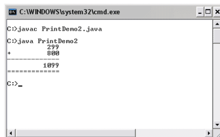
Figure 19: Demonstration of using print() and println() with both String and numeric input
