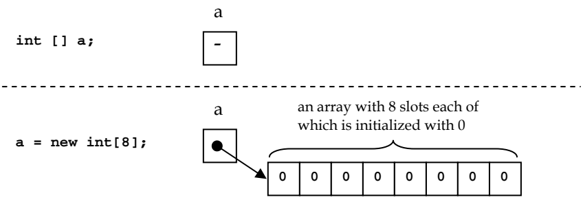
Figure 144: Illustration of memory allocation when a variable is declared and assigned with an array
