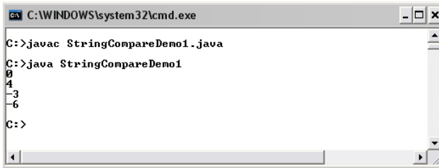
Figure 106: Demonstration showing compareTo() in action
