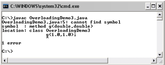
Figure 143: Compilation error due to unmatched overloaded methods
