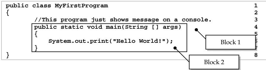
Figure 17: Blocks visualization in MyFirstProgram.java
