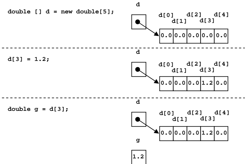
Figure 145: Illustration of accessing an array element
