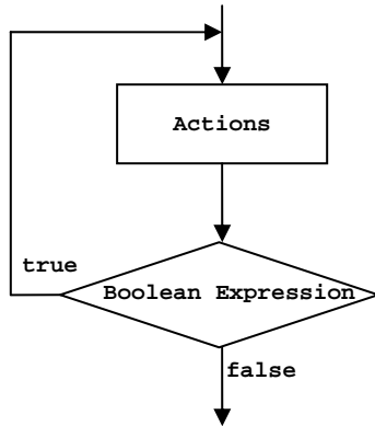
Figure 112: A flowchart representing a do-while statement
