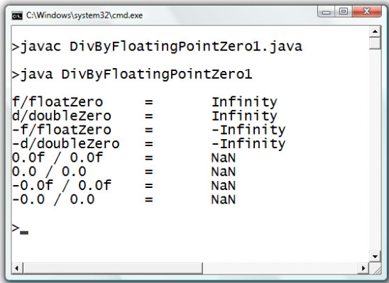
Figure 64: A Java program with expressions evaluated to the double-valued Infinity, -Infinity and NaN
