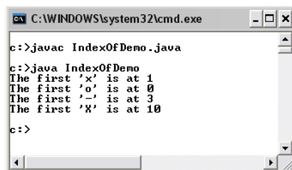
Figure 74: Demonstration of using indexOf()
