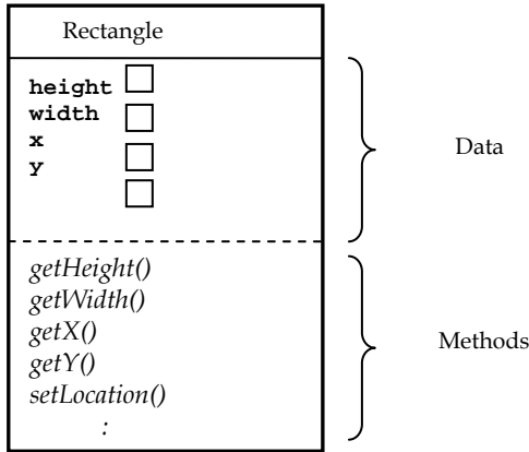
Figure 69: An abstract representation of the details of a class
