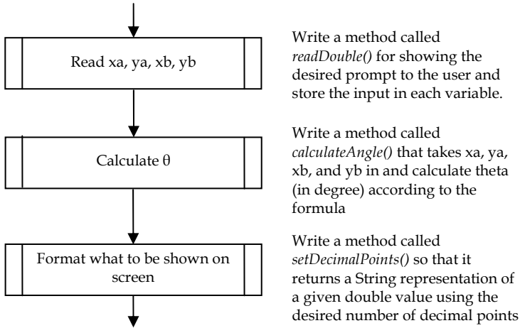
Figure 131: A flowchart showing various subroutines used in the VectorAngle program
