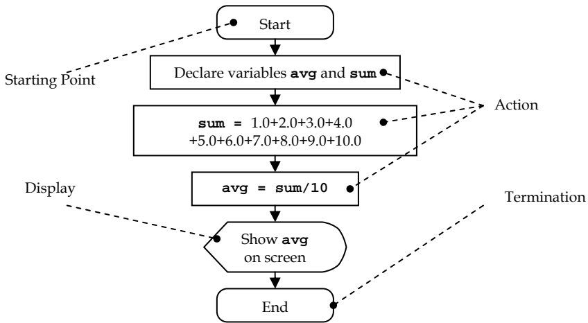
Figure 28: The flowchart of the AverageDemo program
