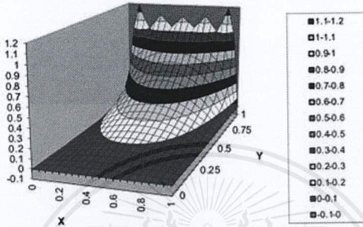
Figure 5. Raised Contour Plot of Analytical Solution (9 terms) Evaluated on a 21x21 Grid
