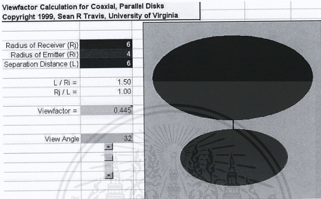
Figure 8. Excel worksheet for viewfactor for coaxial, parallel disks
