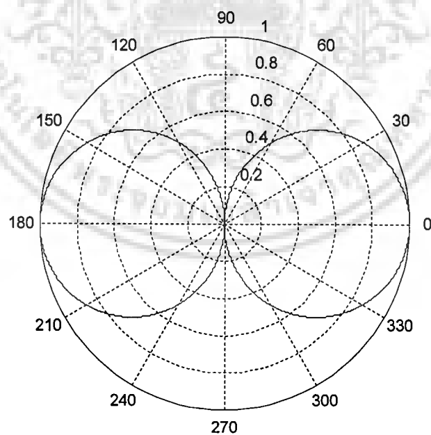
รูป 2.5 directivity pattern of hypercardoid speaker
