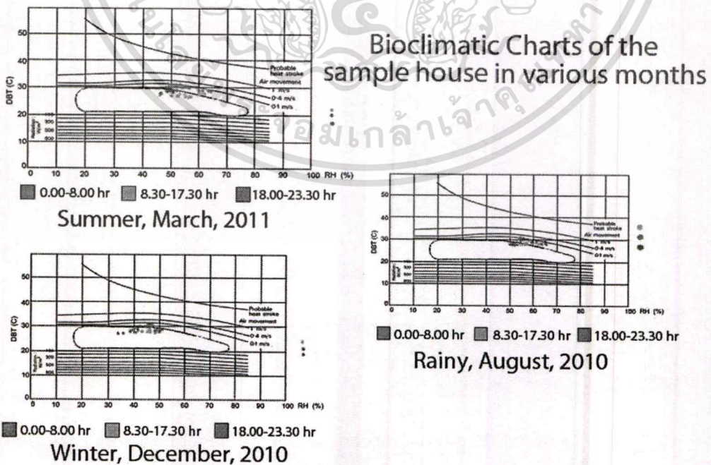
Figure 10: Illustration of Bioclimatic charts of studio room at the sample house
