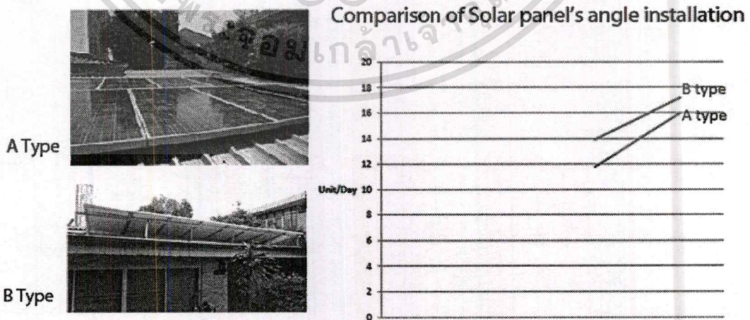
Figure 12: Comparison chart for electrical energy generated from solar panels with inclination at 5 degrees' North (A type) producing electricity of 12-15 unit/day, and solar panels with inclination at 15 degrees' South (B type) producing electricity of 14-17unit/day.
