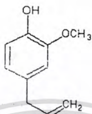
Eugenol
