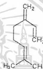
\beta -Myrcene
