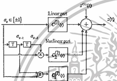
Fig. 7. The second-order Volterra Model for nonlinear transfer response.
