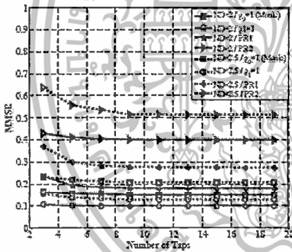
Fig. 8. The MMSE vs. the number of equalizer taps in the nonlinear channel.
