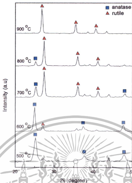
Figure. 3 XRD patterns of \text{TiO}_2 nanofibers calcined at different temperatures.
