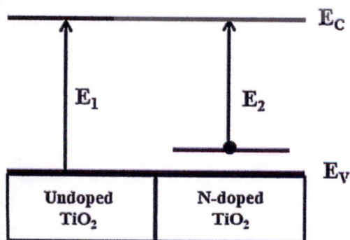
Figure 9 The electronic band structure schematic of the presence of nitrogen in TiO 2 matrix.
