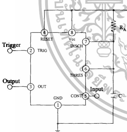
Figure 9. Circuit for Pulse Width Modulation
