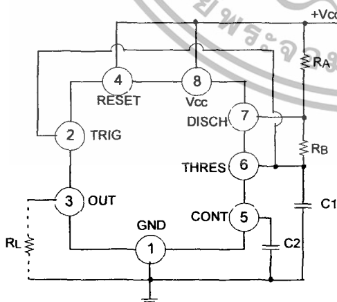
Figure 5. Astable Circuit
