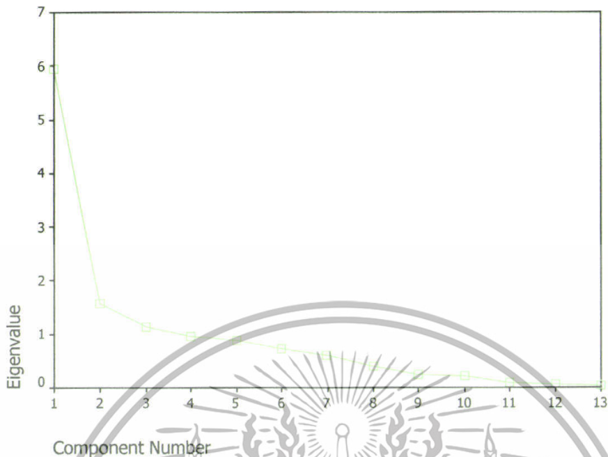
Scree Plot
