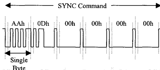
Figure 4 – RS-232 SYNC command timing diagram
