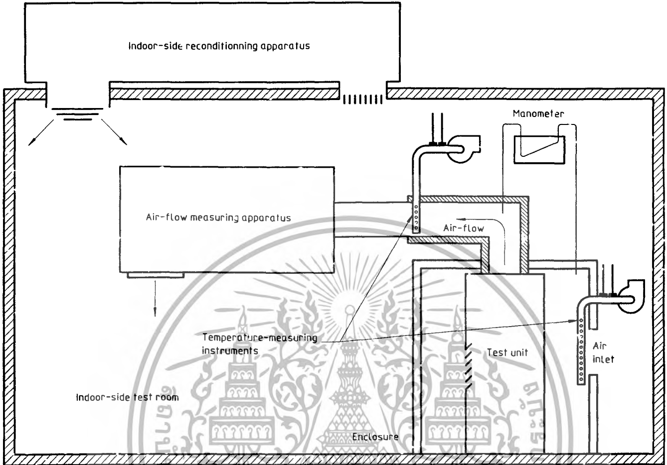
Figure E.1 — Calorimeter: Air-enthalpy test method arrangement
