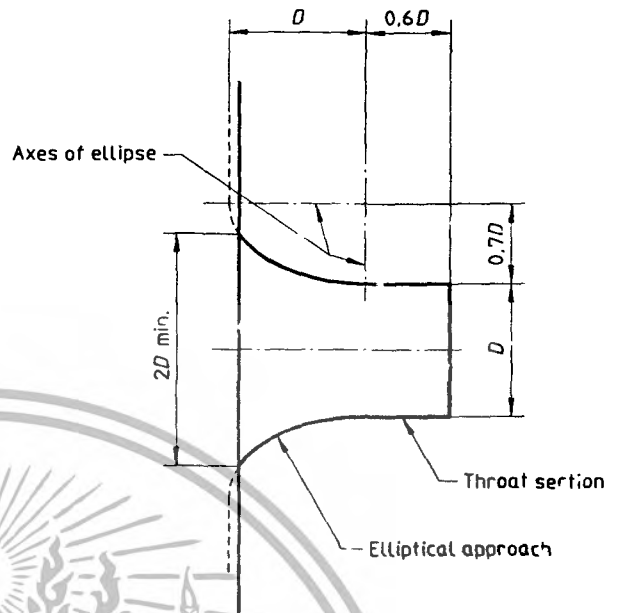
Figure B.2 — Air-flow measuring nozzle
