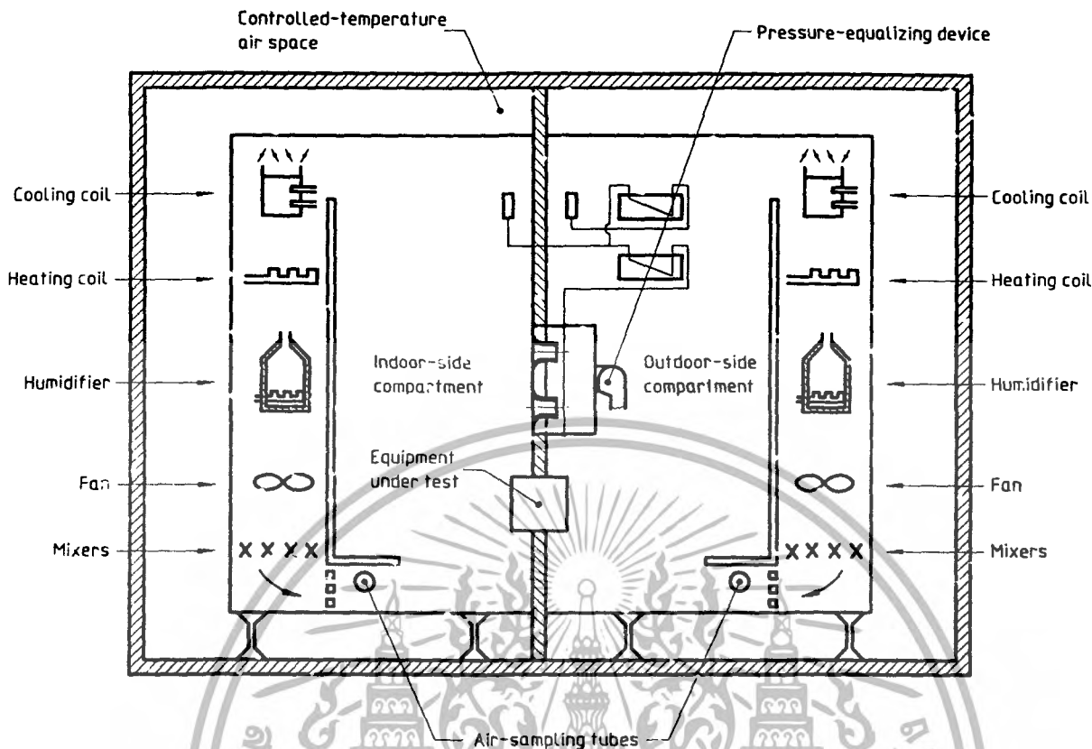
Figure B.5 — Typical balanced ambient room-type calorimeter
