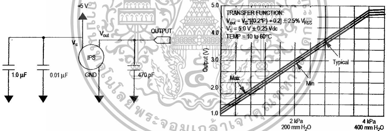
Figure 3. Recommended Power Supply Decoupling and Output Filtering.
