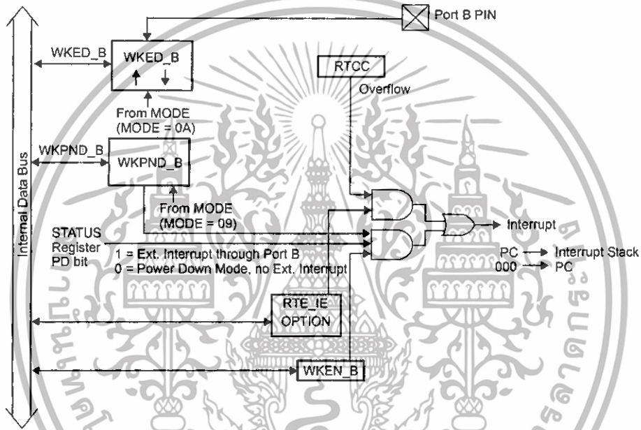
Figure 8-1. Interrupt Structure
