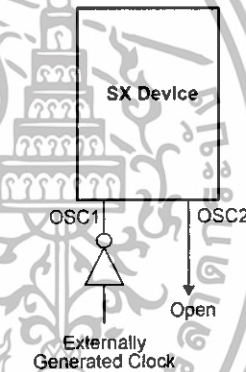
Figure 9-2. External Clock Input Operation (HS, XT or LP OSC Configuration)
