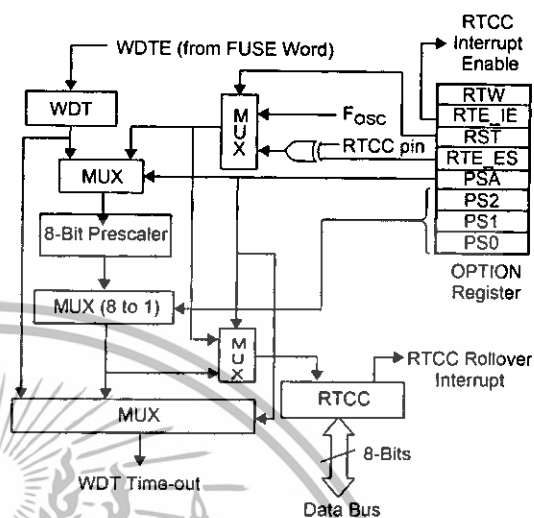
Figure 10-1. RTCC and WDT Block Diagram
