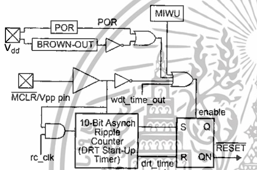
Figure 12-1. Block Diagram of On-Chip Reset Circuit
