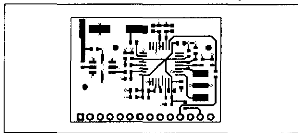
FIGURE 3: rRXD0420 TOP COPPER
