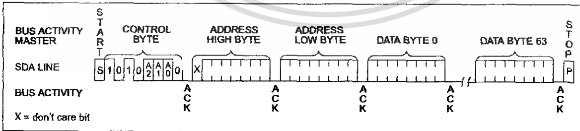
FIGURE 6-2: PAGE WRITE
