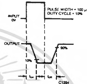
Fig. 11. Switching Time Waveforms
