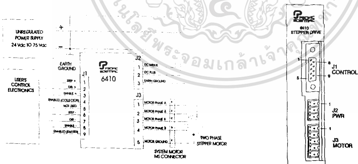
Figure 1 - 6410 Connection Diagram
