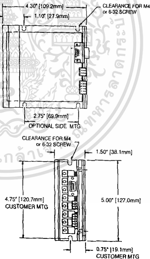
Figure 5 - Mounting Dimensions
