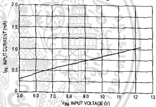
Figure 11. ULN2804 Input Current versus Input Voltage
