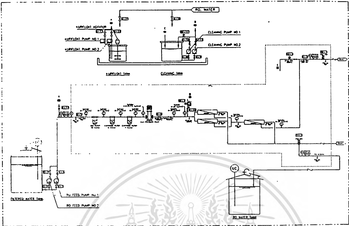
Fig. 5: Automation Reverse Osmosis System
