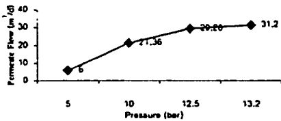
Fig.3: Effect of Pressure on Pure Water
