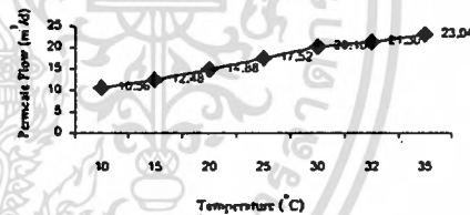
Fig.2: Temperature of Pure water from System
