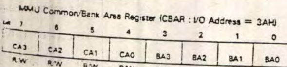
Figure 29. MMU Common/Bank Area Register (CBAR : I/O Address = 3AH)
