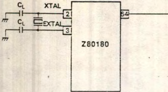
Figure 84. Clock Generator Circuit
