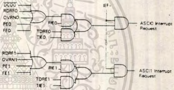
Figure 66. ASCII Interrupt Request Circuit Diagram
