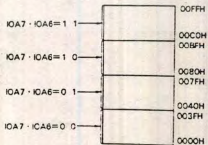
Figure 22. I/O Address Relocation
