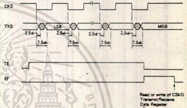
Figure 72. Transmit Timing-External Clock
