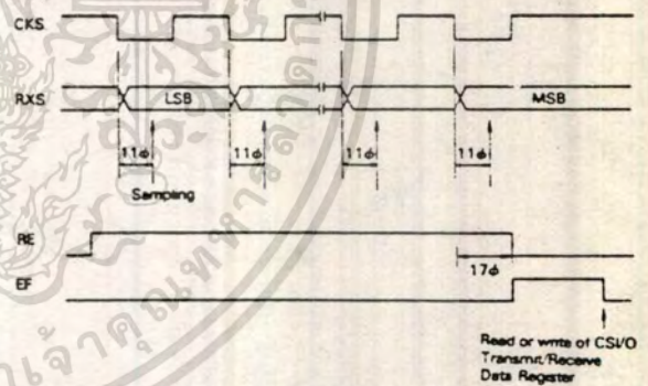
Figure 73. Receive Timing-Internal Clock
