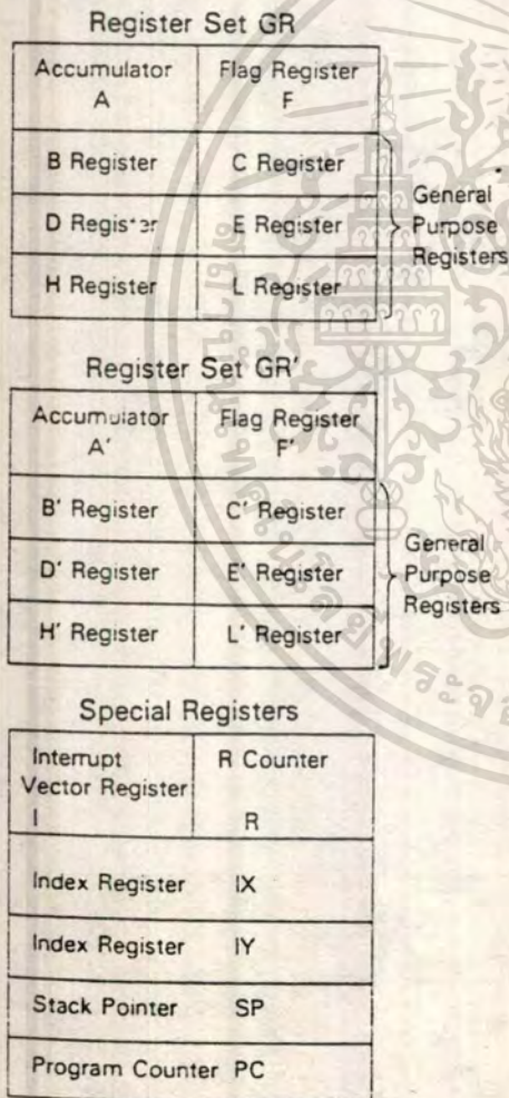
Figure 87. CPU Registers
