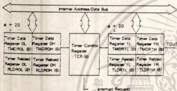
Figure 75. PRT Block Diagram
