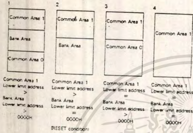
Figure 27. Logical Memory Organization
