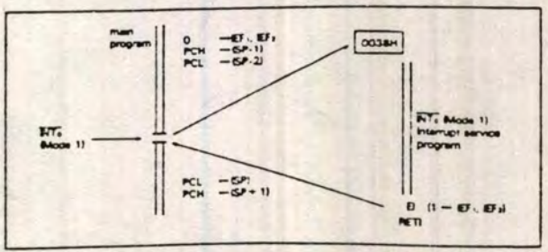
Figure 41. \overline{\text{INT}}_0 Mode 1 Interrupt Sequence
