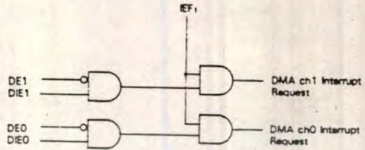
Figure 58. DMA Interrupt Request Generation
