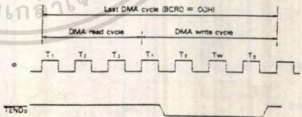
Figure 57. TEND0 Output Timing
