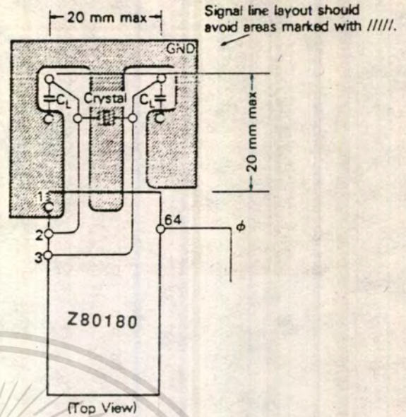
Figure 86. Example of Board Design
