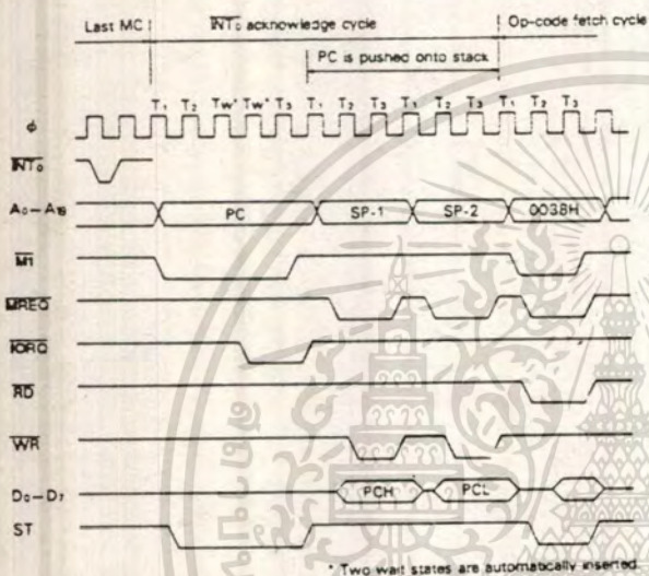
Figure 42. \overline{INT}_0 Mode 1 Timing
