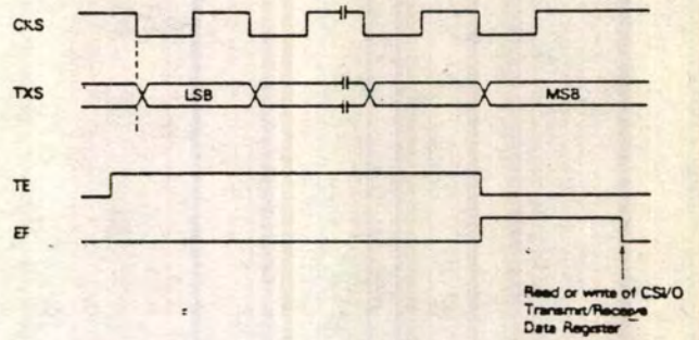
Figure 71. Transmit Timing-internal Clock
