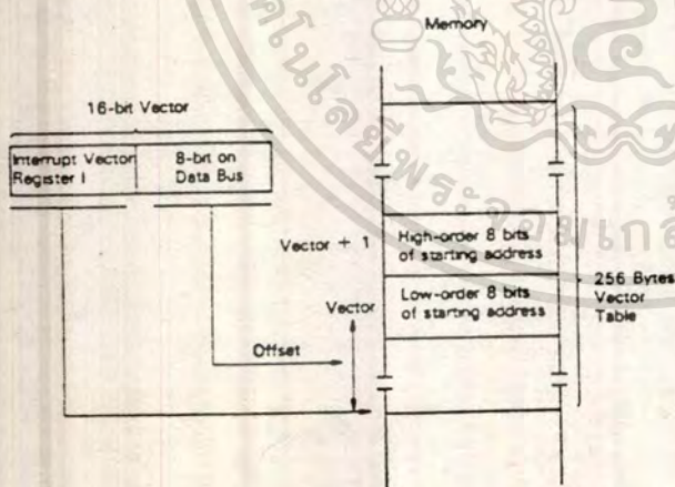
Figure 43. \overline{INT}_0 Mode 2 Vector Acquisition
