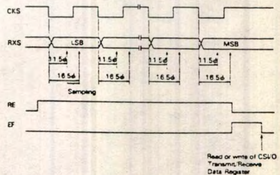
Figure 74. Receive Timing-External Clock
