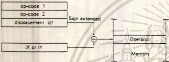
Figure 91. Indexed Addressing
