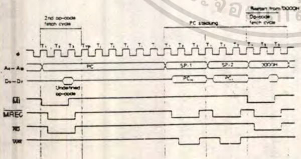
Figure 36. TRAP Timing-2 nd Op-Code Undefined
