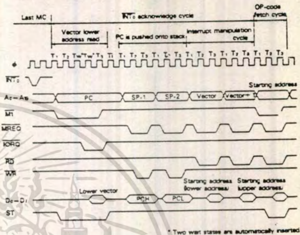
Figure 44. \overline{INT}_0 Interrupt Mode 2 Timing
