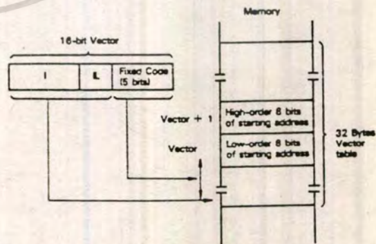
Figure 45. \overline{INT}_1, \overline{INT}_2 Vector Acquisition
