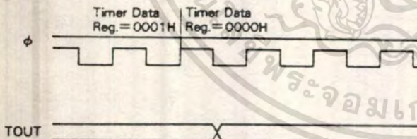
Figure 78. Timer Output Timing
