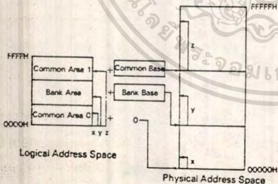
Figure 24. Physical Address Translation
