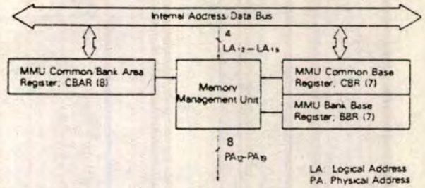
Figure 25. MMU Block Diagram
