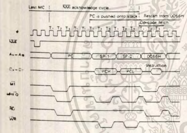
Figure 39. \overline{\text{NMI}} Timing
