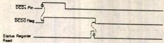
Figure 64. \overline{DCD}_0 Timing
