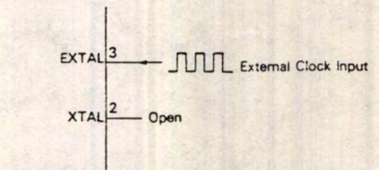
Figure 83. External Clock Interface
