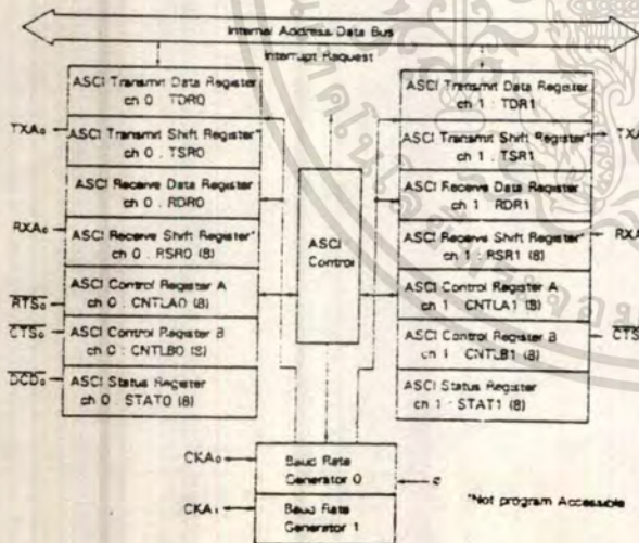
Figure 50. ASCI Block Diagram
