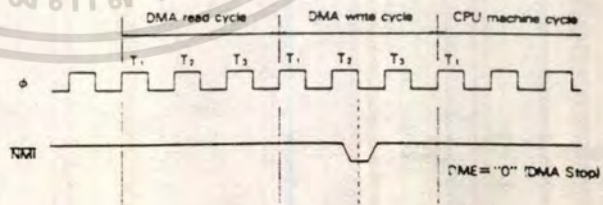
Figure 59. NMI and DMA Operation
