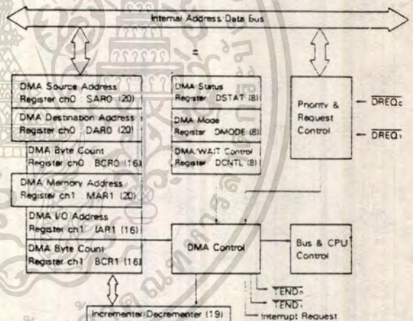
Figure 50. DMAC Block Diagram
