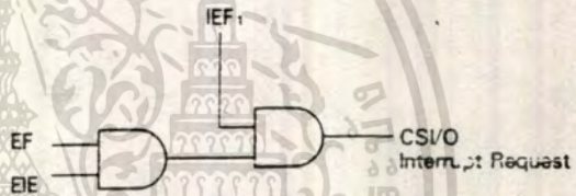
Figure 70. CSI/O Interrupt Request Generation
