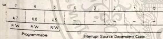
Figure 34. Interrupt Vector Low Register (IL : I/O Address = 33H)
