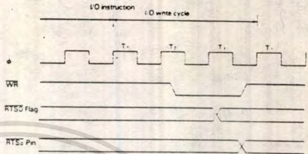
Figure 65. \overline{RTS}_0 Timing
