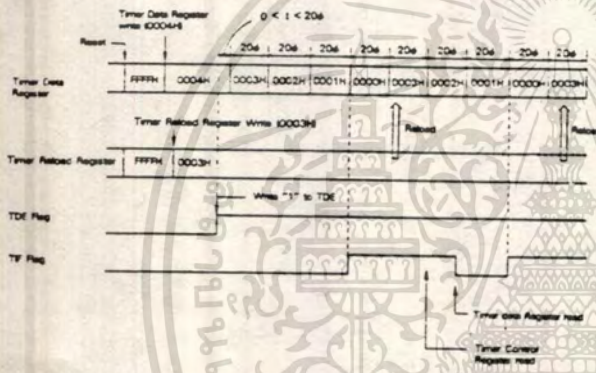
Figure 77. Timer Initialization, Count Down, and Reload Timing
