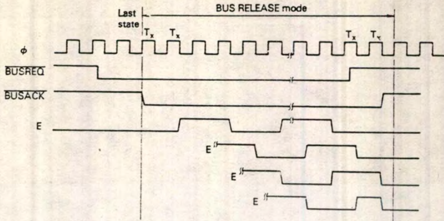
Figure 81. E Clock Timing in BUS RELEASE Mode
