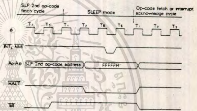
Figure 20. SLEEP Timing
