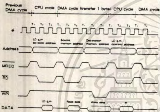
Figure 54. DMA Timing-Cycle Steal Mode
