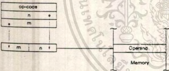
Figure 92. Extended Addressing
