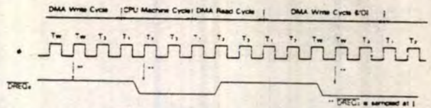
Figure 55. CPU Operation and DMA Operation (DREQ0 is Programmed for Level Sense)
