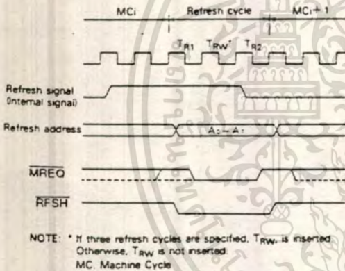
Figure 48. Refresh Cycle Timing
