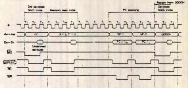
Figure 37. TRAP Timing-3 rd Op-Code Undefined
