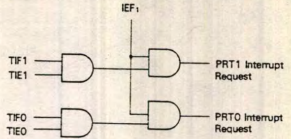
Figure 79. PRT Interrupt Request Generation
