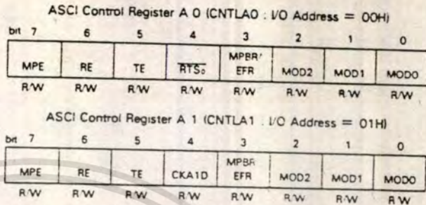
Figure 62. ASCII Control Register A
