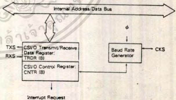
Figure 68. CSI/O Block Diagram
