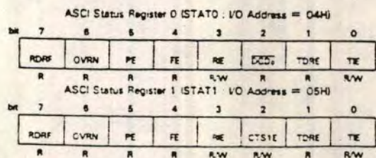
Figure 61. ASCI Status Registers
