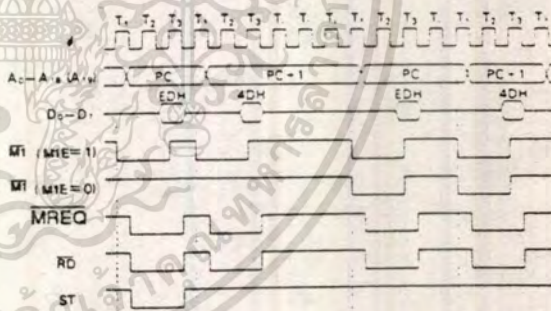
Figure 47. RETI Instruction Sequence
