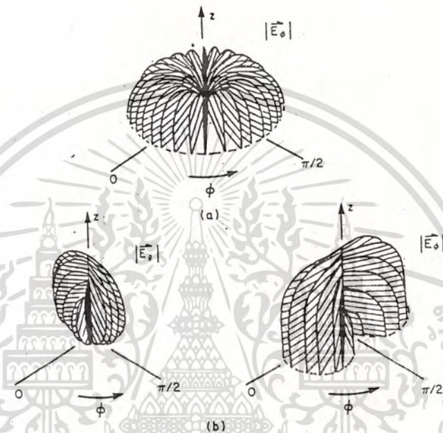
FIG2-6-16 Far-zone electric field patterns in upper hemisphere. (a) Electrically small loop, \beta b \ll 1 . (b) Resonant loop, \beta b = 1.0 .
