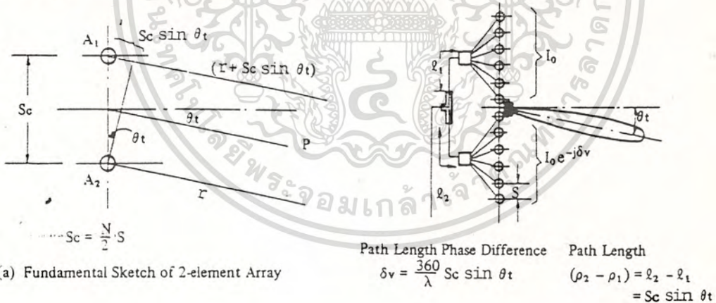
Fig. 2.4 Beam Tilting of a N-element Array
