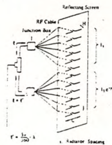
Fig. 3.16 Configuration of 12-Radiators
