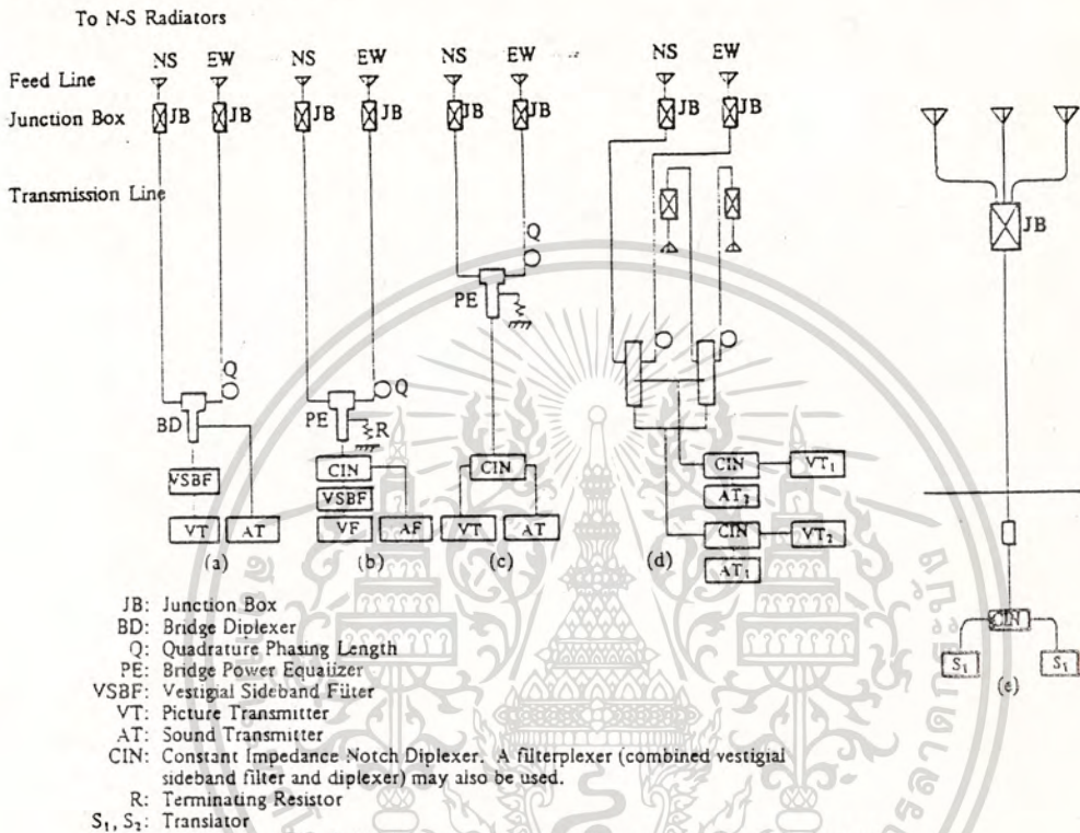
Fig. 2.14 Transmission Line Systems for Feeding Antennas
