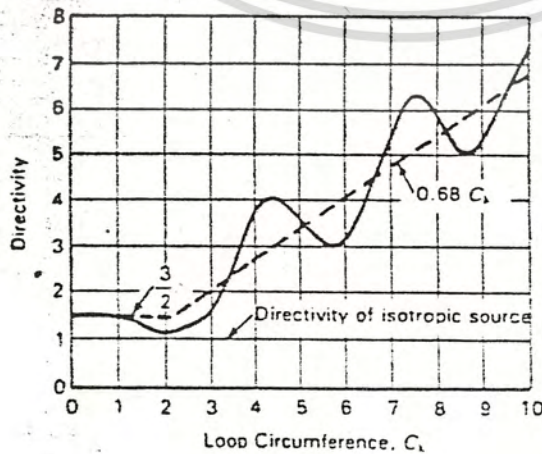
Figure 2-6-7 Directivity of circular loop antenna with uniform, in-phase current as a function of loop circumference in wavelengths, C_1 . (After D. Foster, "Loop Antennas with Uniform Current," Proc. IRE, 32, 603-607, October 1944.)
