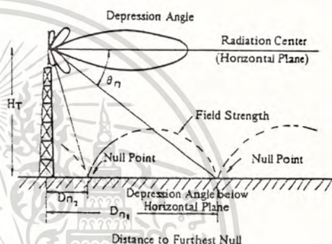
Fig. 2.5 Effect of Vertical Pattern Nulls on Close in Coverage
