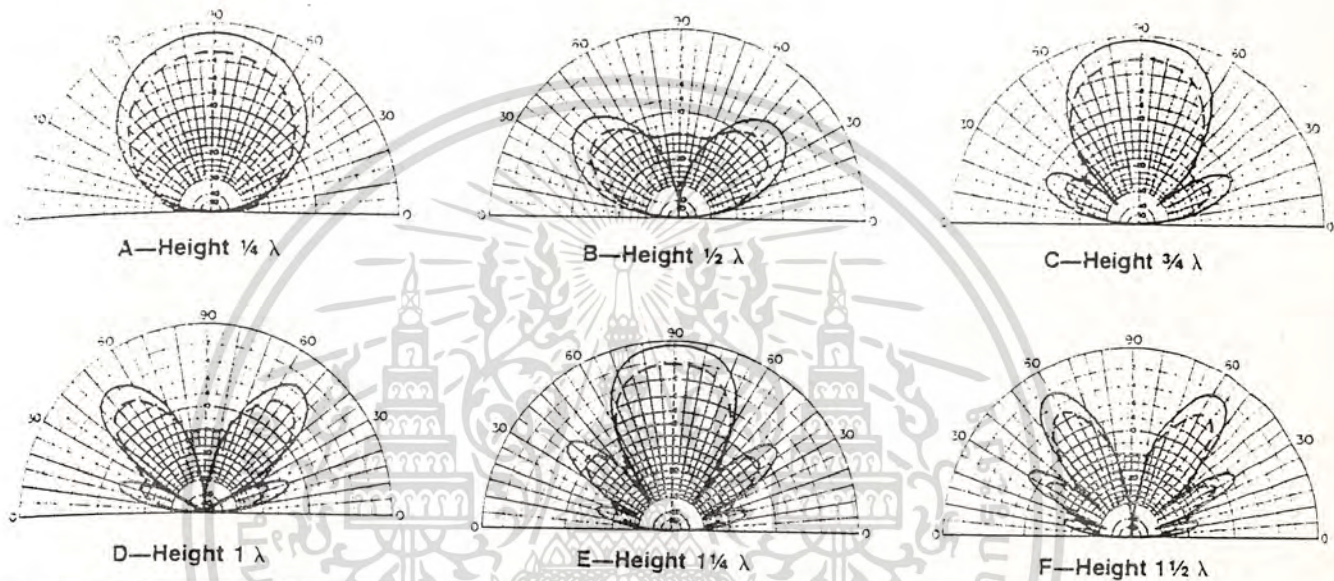
Fig. 11—Vertical-plane radiation patterns of horizontal half-wave antennas in the plane of the antenna wire. The solid-line curves are the perfect-earth patterns, and the shaded curves represent the effects of average earth ( k = 15 , G = 0.005 \text{ S/m} ) at 14 MHz. The 0-dB reference in each plot corresponds to the peak of the main lobe in the favored direction of the antenna (the maximum gain). Add 6 dB to values shown.
