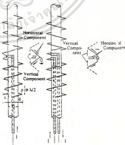
Fig. 3.26 (a) Side-Fire Helical Antenna
