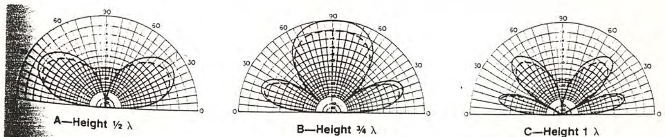
Fig. 12—Vertical-plane radiation patterns of half-wave horizontal antennas at 45^\circ from the antenna wire. The solid-line curves represent the same conditions as in Figs 11 and 12. These patterns are scaled so they may be read directly with those of Figs 11 and 12.
