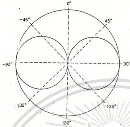
FIGURE Relative radiation pattern for an elementary doublet in a plane perpendicular to the dipole axis.
