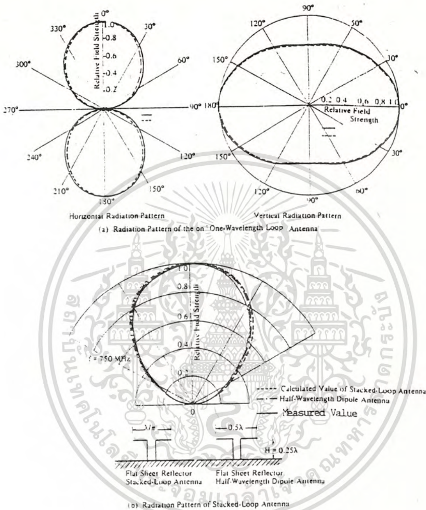
Fig. 3.23 Radiation Patterns of Loop-Antenna and Stacked-Loop Antenna
