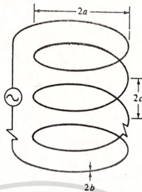
(a) N -turn circular loop
