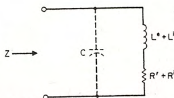
FIG2-623 Equivalent circuit for input impedance Z of an electrically small loop.
