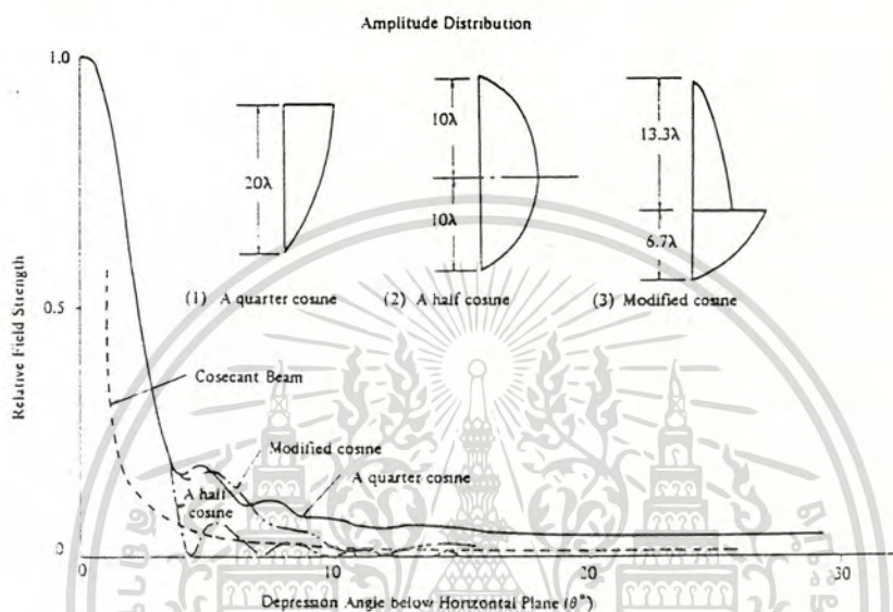
Fig. 2.9 An Example of Null Filling Calculation by Twin-beam Method
