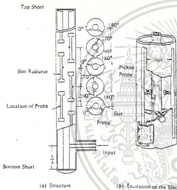
Fig. 3.20 (a) (b) Traveling-Wave Slot Antenna
