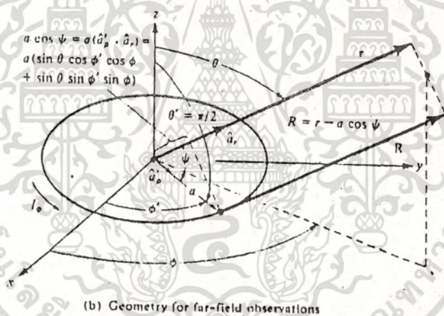
Figure Geometrical arrangement for loop antenna analysis.
