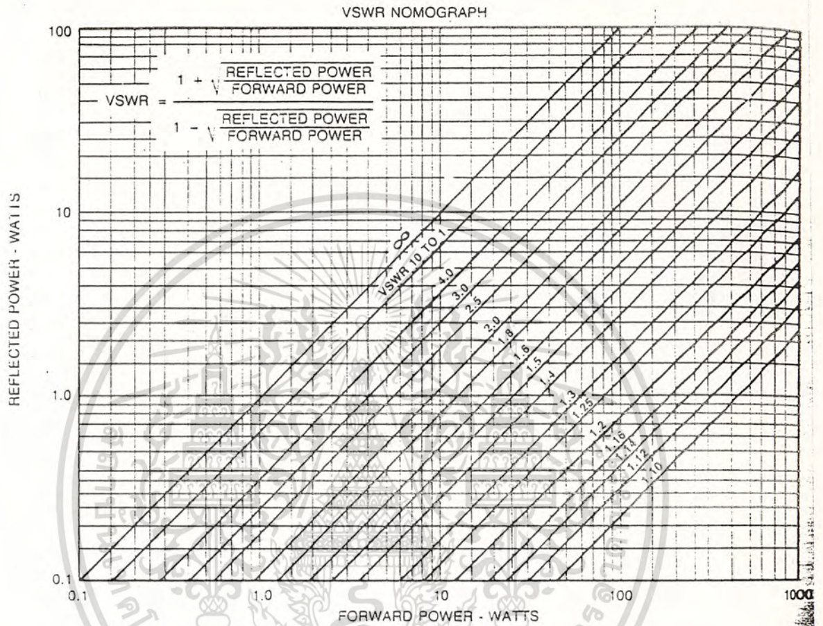
Fig - SWR as a function of forward and reflected power.
