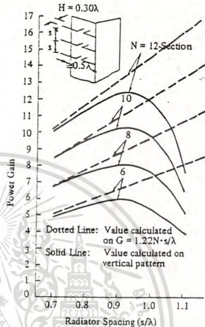
Fig. 3.17 Power Gain of a Super-Gain Antenna
