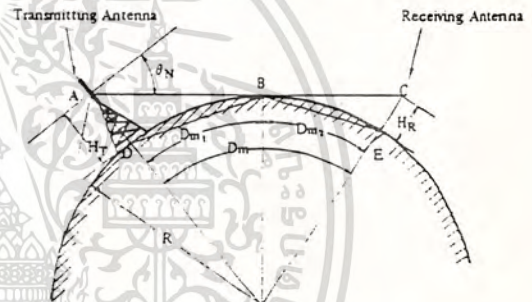
Fig. 2.1 Ray Paths for Antennas above Spherical Earth
