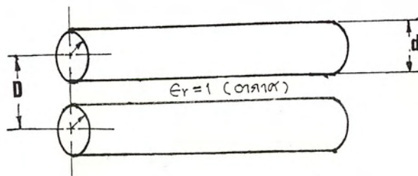
รูป 3-4 Two-Wire Transmission Line
