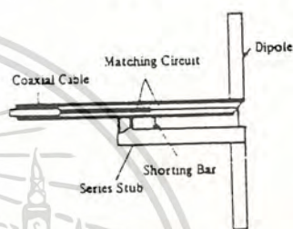
Fig. 3.29 (a) Structure of Driven Element
