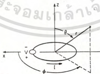
FIG2-5-21 Loop antenna and accompanying spherical coordinate system.
