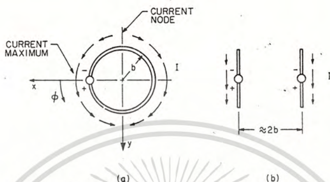
FIG25-14 Schematic of current distribution in resonant loop (a) and in the approximately equivalent pair of dipoles (b).
