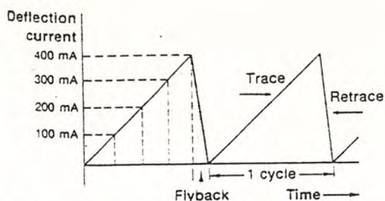
Fig. Sawtooth scanning waveform, used for H and V deflection.
