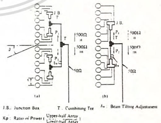
Fig. 2.12 Transmission Line Systems for Feeding Antennas of 12-section Antenna
