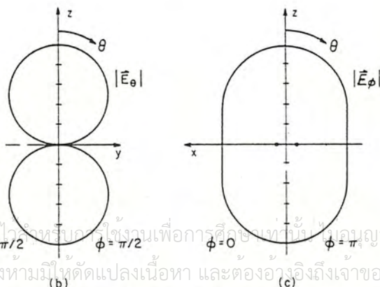
FIG25-15 Far-zone electric field for loop with \beta b = 1.0 , \Omega = 10 . (a) Horizontal-plane field pattern |E_\phi| , \theta = \pi/2 . (b) Vertical-plane field pattern |E_\theta| , \phi = \pi/2 , 3\pi/2 . (c) Vertical-
