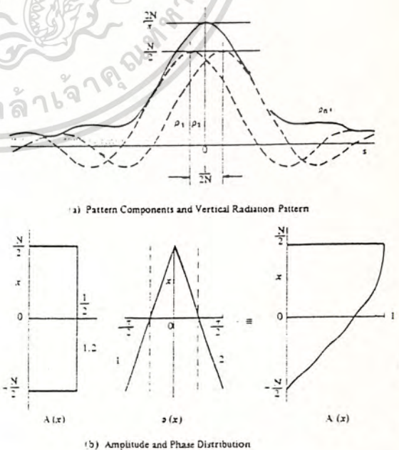
Fig. 2.8 Principles of Twin-Beam Method
