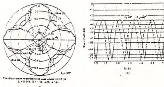
Fig. 3.19 Field Pattern and Worst Null Depth Calculations of an Antenna with 90° Skew
