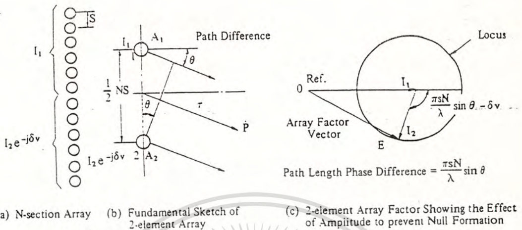
Fig. 2.7 Effect of Current Amplitude Unbalance in Reducing Depth of Vertical Pattern Nulls
