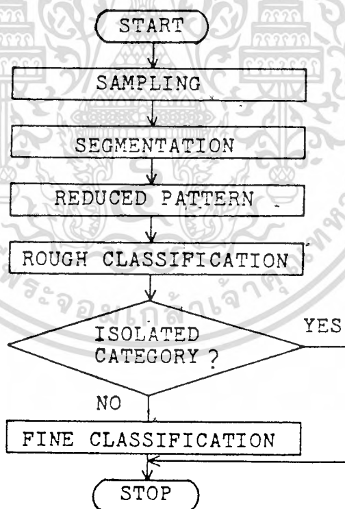
Fig. 8 Sequence of recognition method
