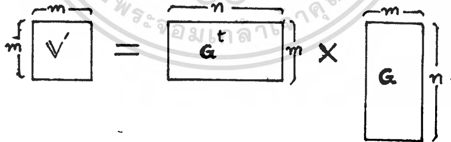
Fig. 18 Dimension of matrix V' = G^T \cdot G
