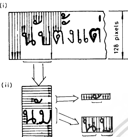
Fig. 8 A method of segmentation
