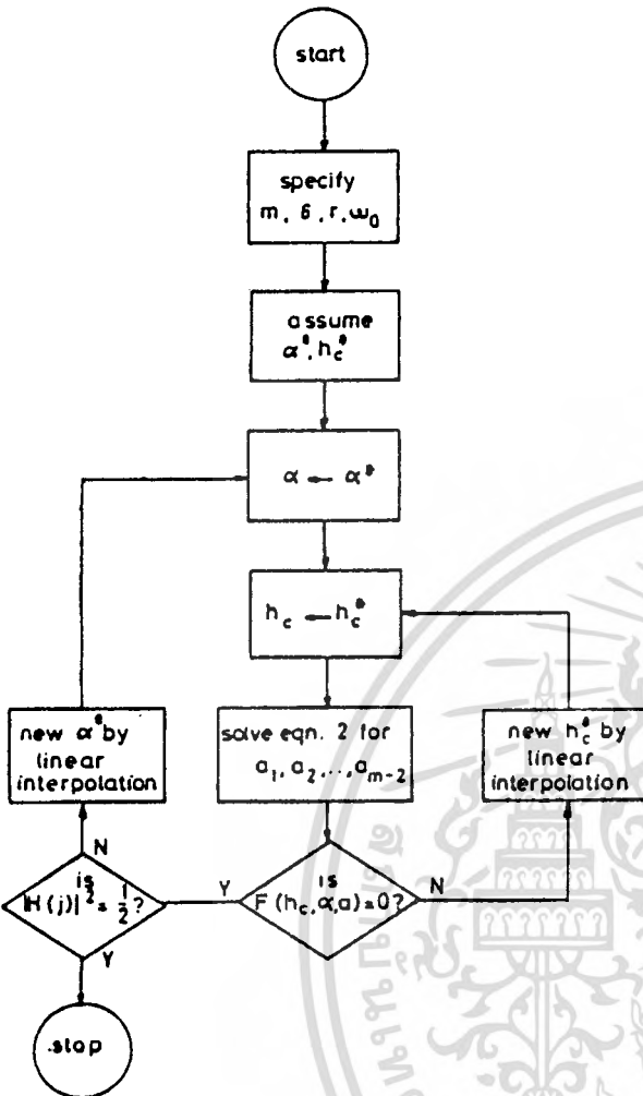
Fig. 1 Flow chart of computer program
