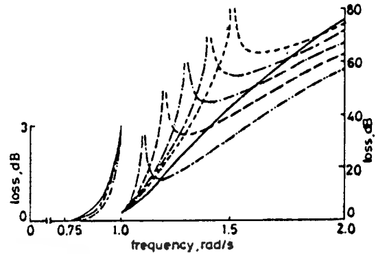
Fig. 2 Responses for m = 10 , \mu_r = 2 , r = 1
