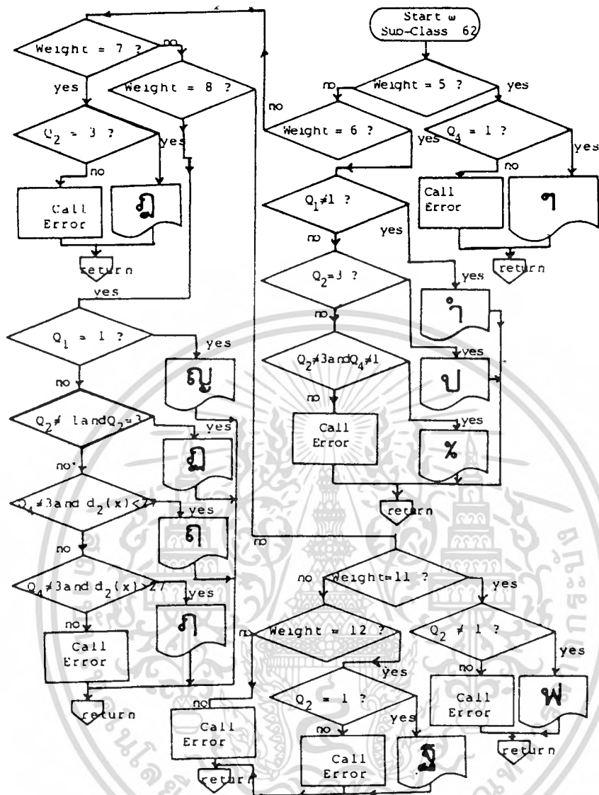
Figure 40 Procedure of the fine classification stage.
