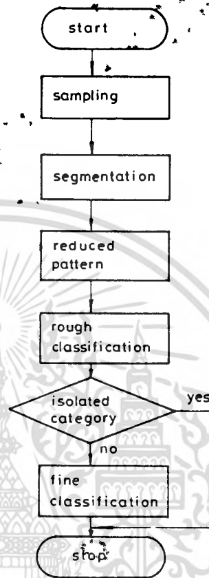
Fig. 7 Sequence of recognition method
