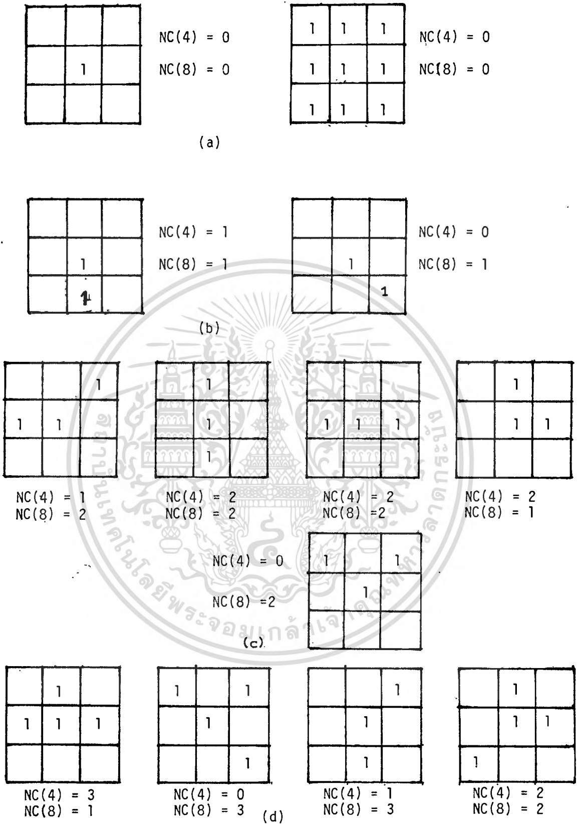
Fig. 36 : (a) NC(4) and NC(8) of independent or inner strokes. (b) NC(4) and NC(8) of end strokes. (c) NC(4) and NC(8) of connecting strokes. (d) NC(4) and NC(8) of branch strokes.
