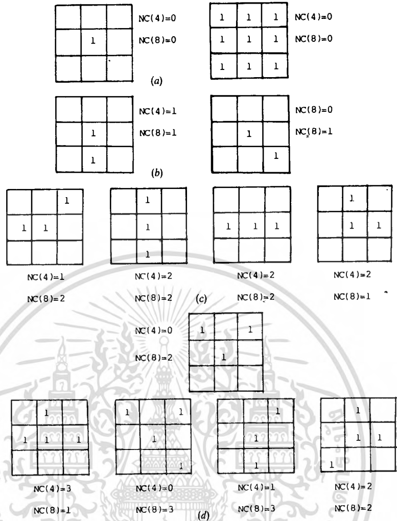
Figure 6. (a) NC(4) and NC(8) of independent or inner strokes. (b) NC(4) and NC(8) of end strokes. (c) NC(4) and NC(8) of connecting strokes. (d) NC(4) and NC(8) of branch strokes.
