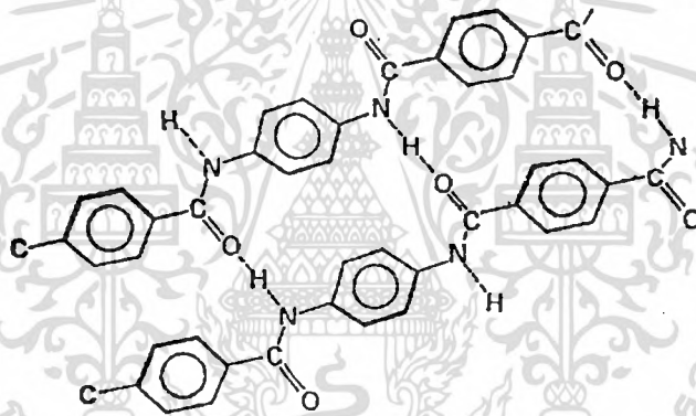
Figure 2.4 Chemical structure of the straight-chain Kevlar showing intermolecular hydrogen bonding (27)
