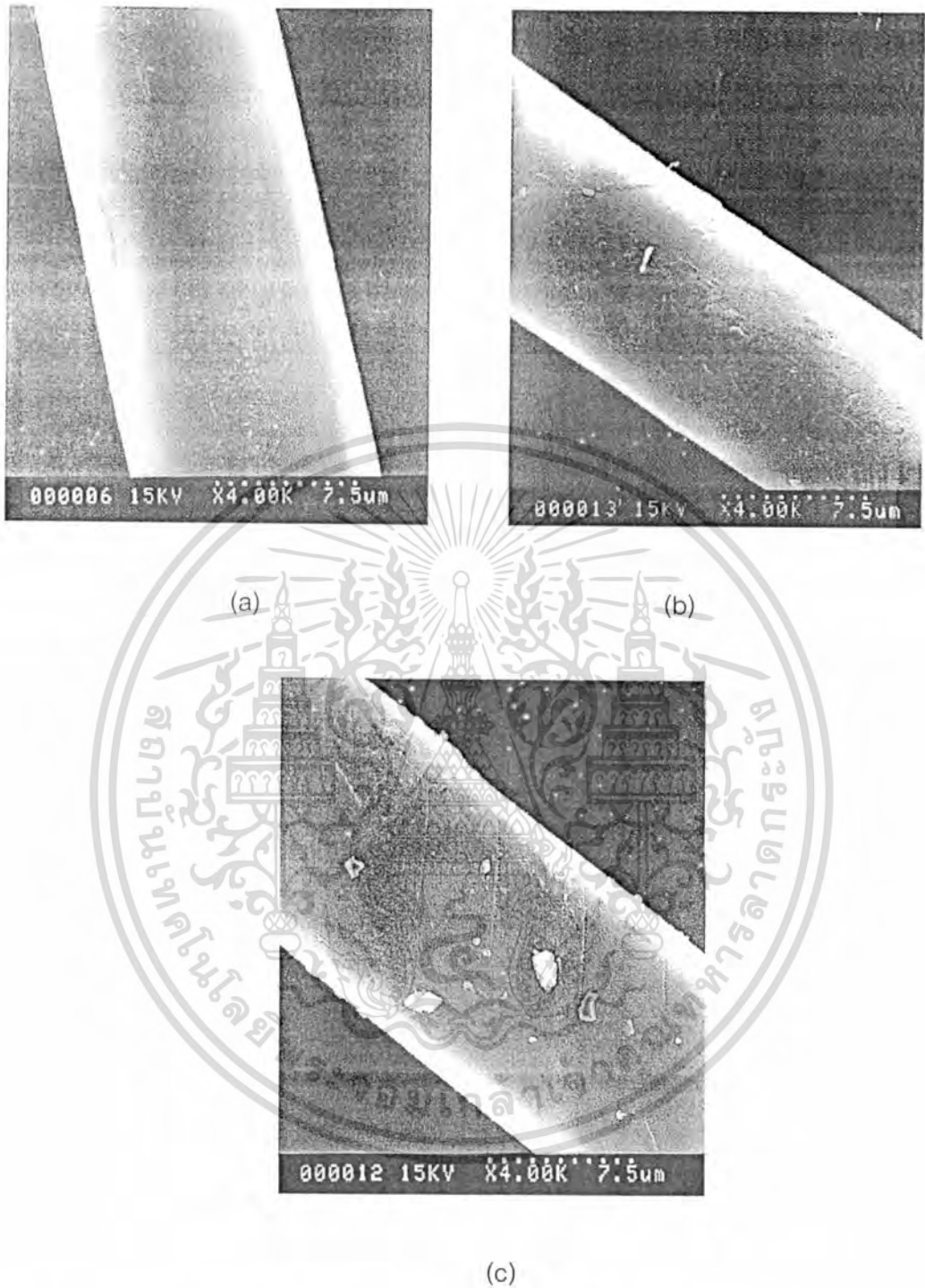
Figure 4.1 SEM micrographs of Kevlar short fibre surfaces :
