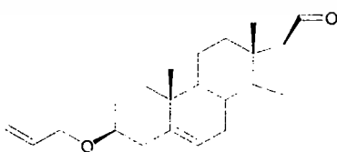
3β-Alloxy-5-pregnene-20-one (118)
