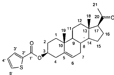
3β-Thiophene-2-carbonate-5-pregnene-20-one (117)
