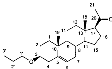
3β-Propoxy-5-pregnene-20-one (119)
