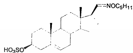
3β-Sulfate-5-pregnene-20-oxime ether (135)
