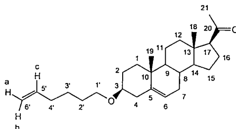
3 \beta -5-ene-Hexoxy-5-pregnene-20-one (121)
