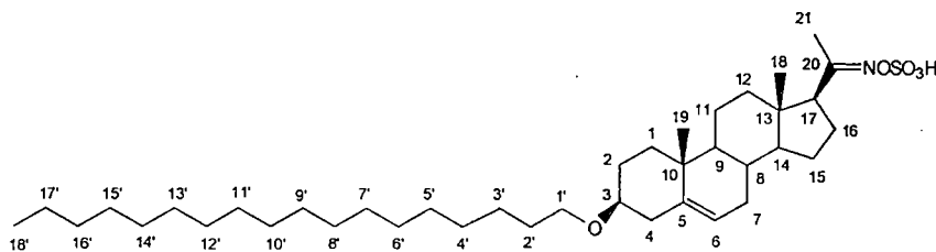
3β-Octadecoxy-5-pregnene-20-oxime sulfonate (143)
