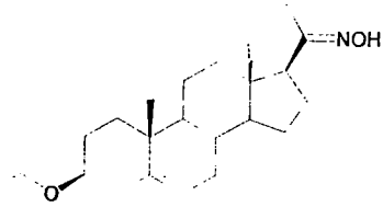
3β-Alloxy-5-pregnene-20-oxime (128)
