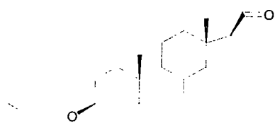
3β-Alloxy-5-pregnene-20-one (118)
