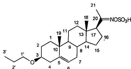
3β-Propoxy-5-pregnene-20-oxime sulfonate (139)
