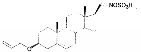
3β-Alloxy-5-pregnene-20-oxime sulfonate (138)
