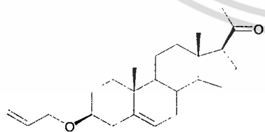
3β-Alloxy-5-pregnene-20-one (118)
