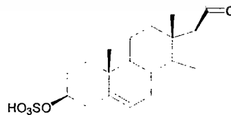
3β-Sulfate-5-pregnene-20-one (124)
