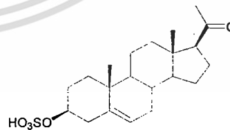
3β-Sulfate-5-pregnene-20-one (124)
