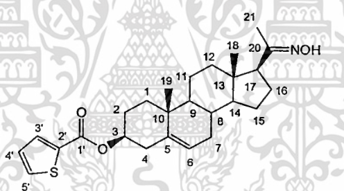
3β-Thiophene-2-carboxylate-5-pregnene-20-oxime (127)
