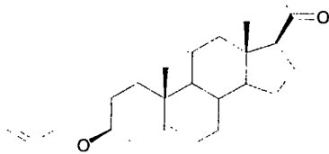
3β-Alloxy-5-pregnene-20-one (118)
