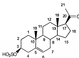
3β-Sulfate-5-pregnene-20-one (124)
