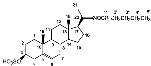
3β-Sulfate-5-pregnene-20-oxime ether (135)
