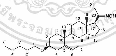
3 \beta -Pentoxy-5-pregnene-20-oxime (130)
