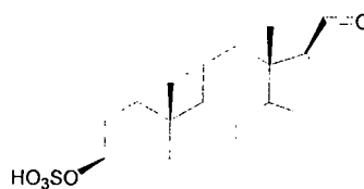
3β-Sulfate-5-pregnene-20-one (124)
