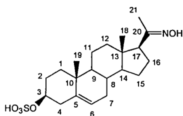
3 \beta -Sulfate-5-pregnene-20-oxime (134)
