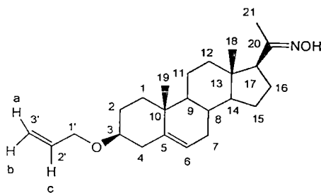
3β-Alloxy-5-pregnene-20-oxime (128)
