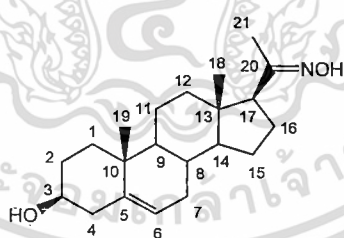
3 \beta -Hydroxy-5-pregnene-20-oxime (125)
